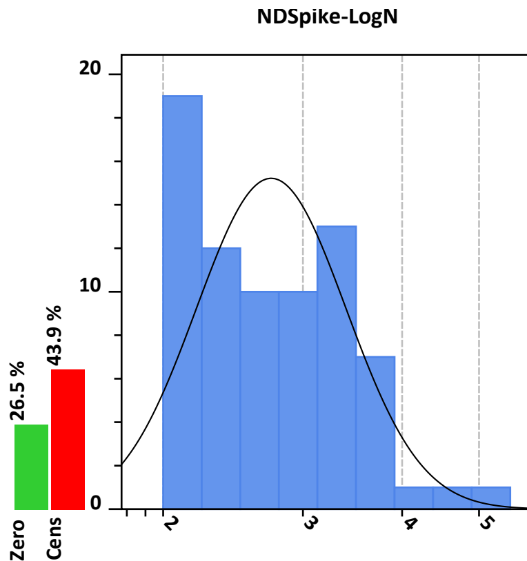
Figure 3.10: Nondetect Spike Lognormal distribution
