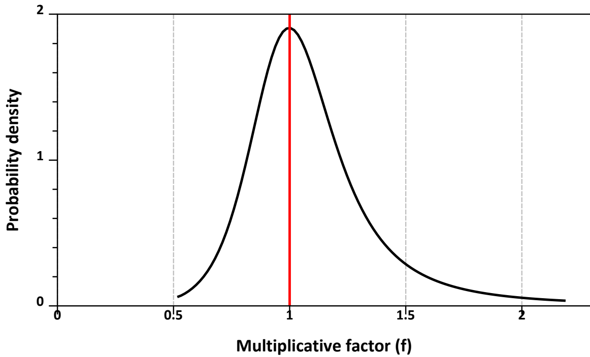
Figure 3.56: Scaled logstudents t ( \mu = -0.593 , s = 0.367 , \nu = 3 , offset=0.5), table 9, [EFSA (2020b)].
