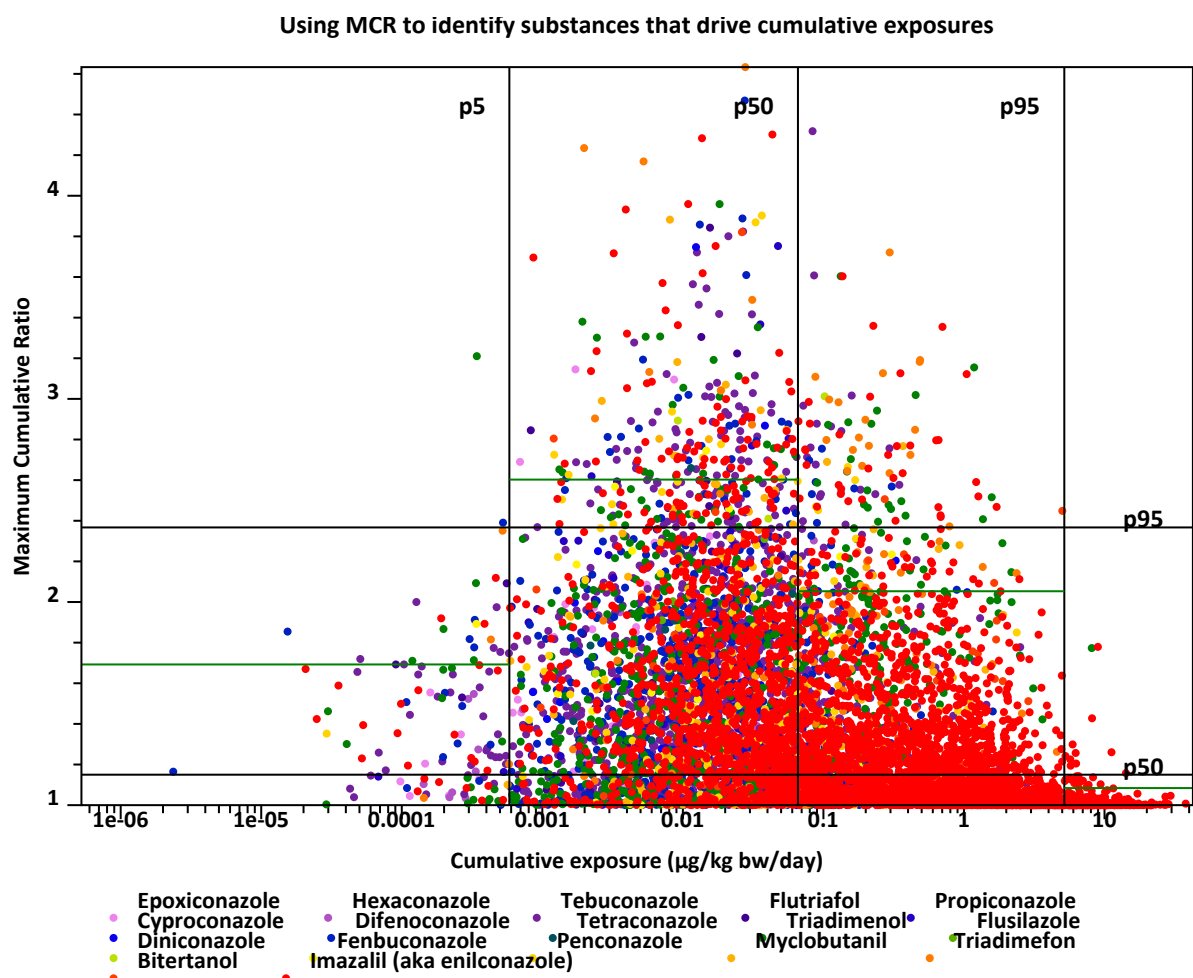
Figure 3.33: Maximum Cumulative Ratios vs total exposure
