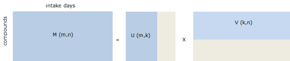
Figure 3.38: NMF approximation of exposure data
