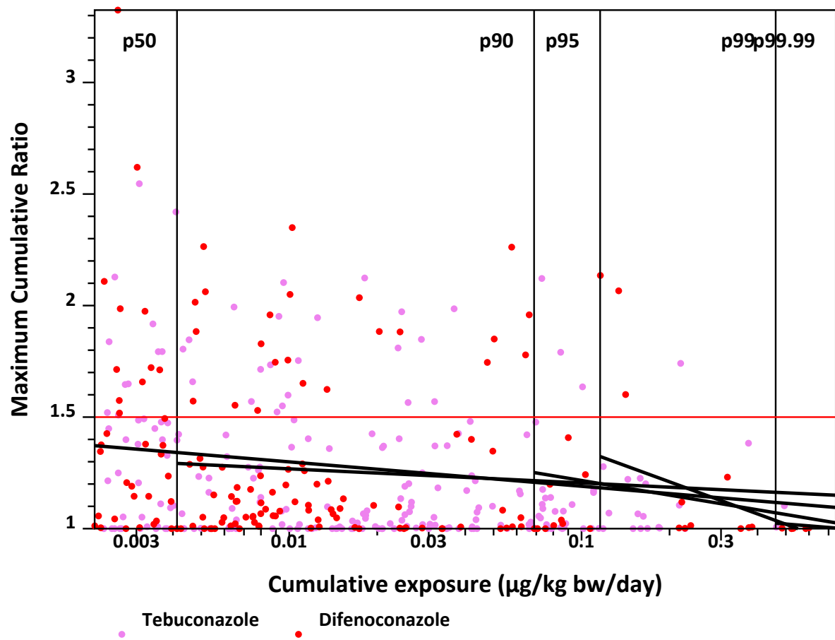
Figure 3.36: Using MCR to identify substances that drive cumulative exposures, scatter distributions (upper tail 37%).
