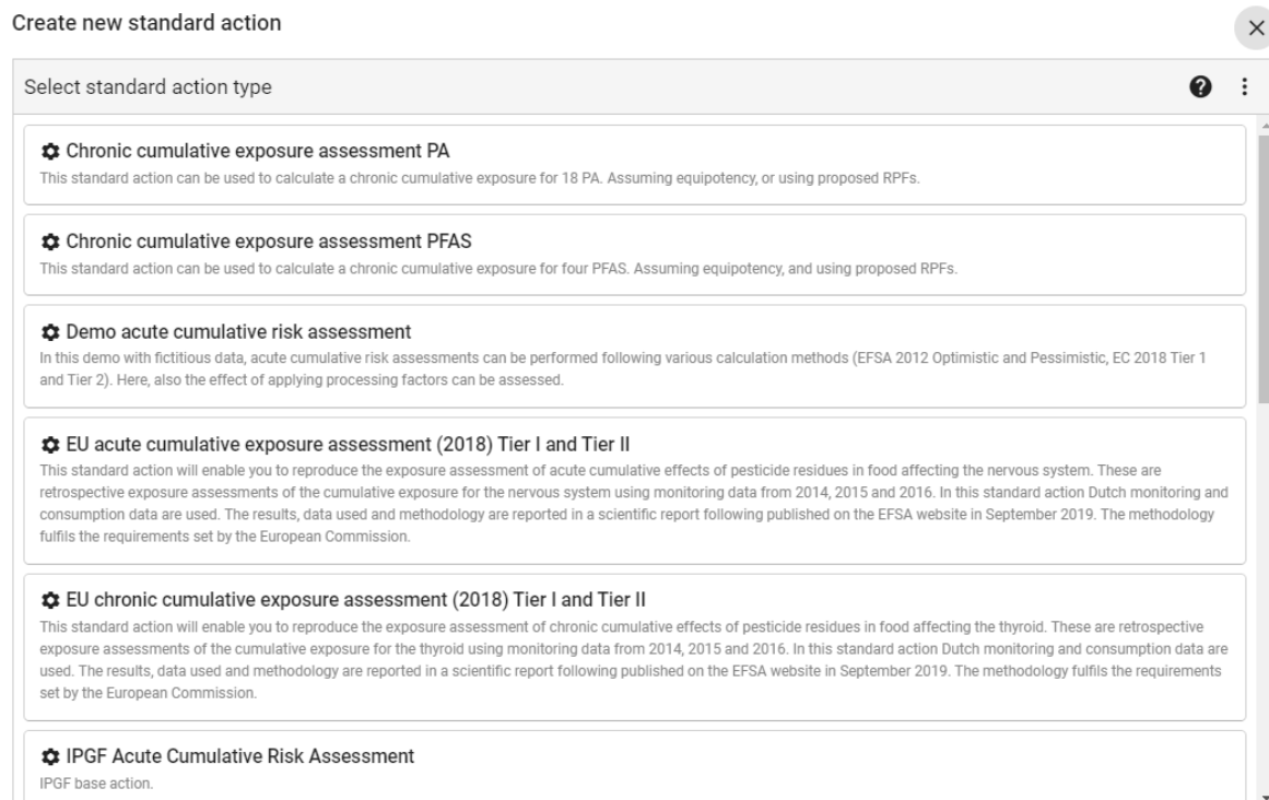
Figure 1.15: Create standard action.
