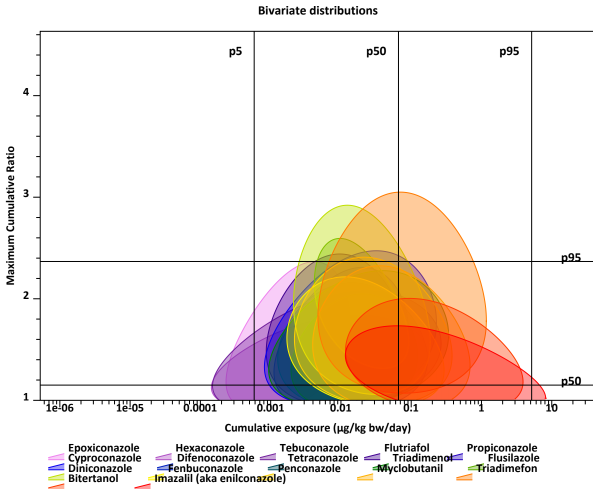
Figure 3.34: Bivariate distributions MCR vs total exposure
