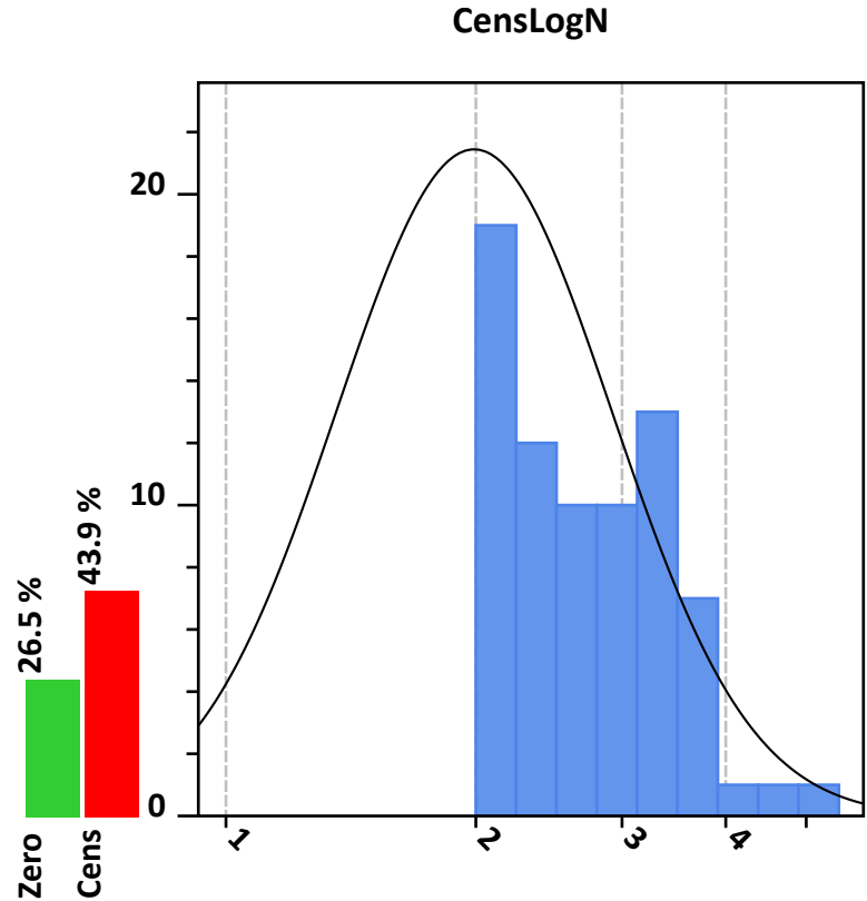
Figure 3.12: Censored Lognormal distribution
