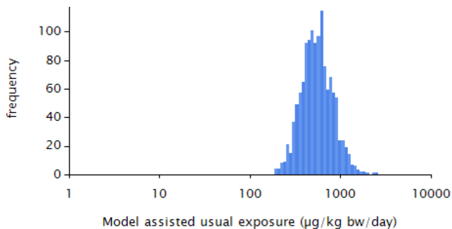
Figure 3.28: Model-based estimated usual exposure distributions (excluding the zero exposures).
