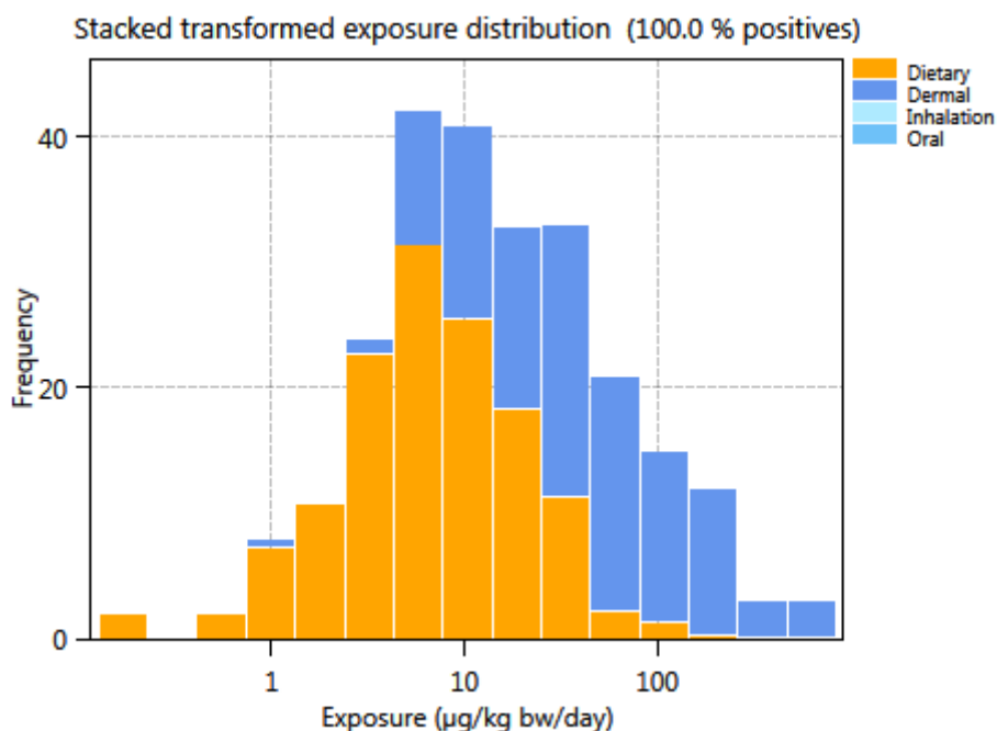
Figure 3.29: Aggregate exposure distributions.
