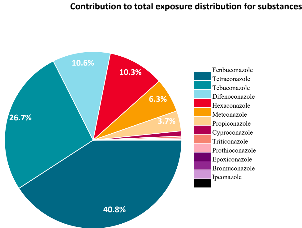
Figure 3.21: Example MCRA dietary exposure contributions foods as eaten
