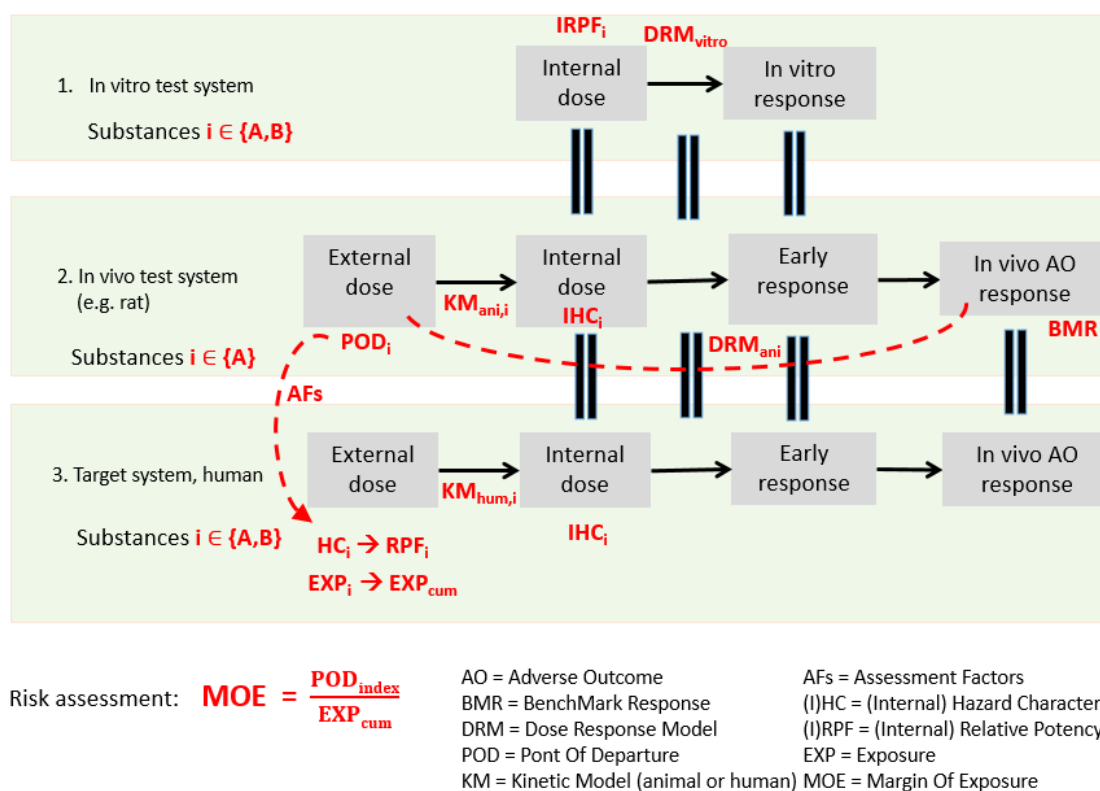
Figure 3.48: Conceptual model IVIVE.
