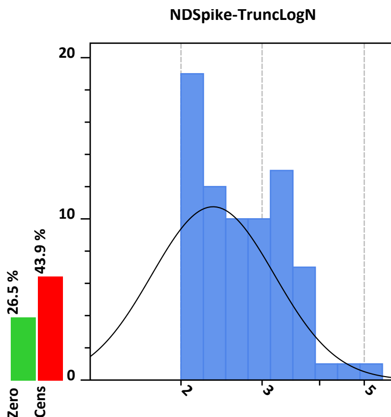
Figure 3.11: Nondetect Spike Truncated Lognormal distribution
