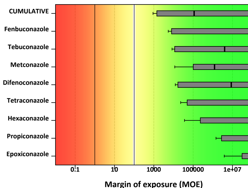
Figure 3.53: Individual margin of exposure (MOE) plot for multiple substances.
