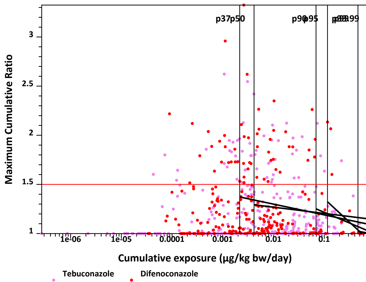
Figure 3.35: Using MCR to identify substances that drive cumulative exposures, scatter distributions (total).
