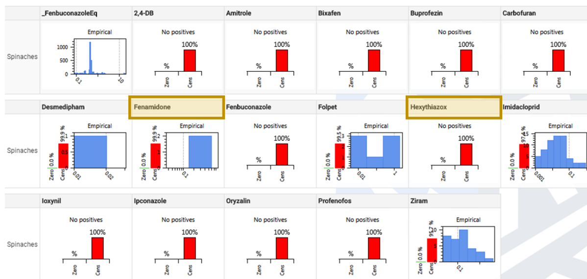
Figure 3.15: All non-detects are replaced by a constant factor \times LOR. For Fenamidine and Hexythiazox (brown boxes) authorized use is assumed.
