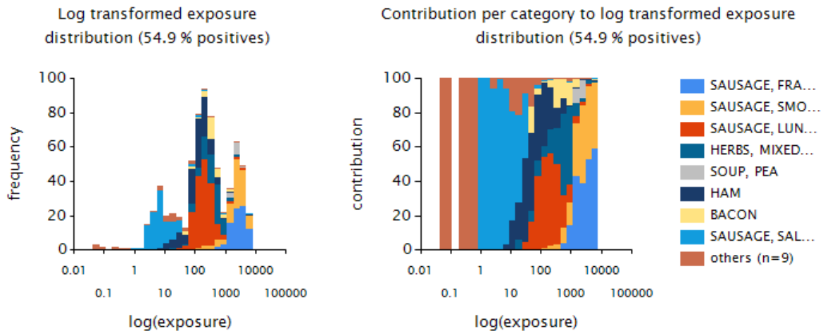
Figure 3.24: Left panel: OIM usual exposure distribution to smoke flavours via the different foods (excluding the zero exposures) in young children; right panel: Contribution of foods to exposures within each bar of the OIM distribution histogram.
