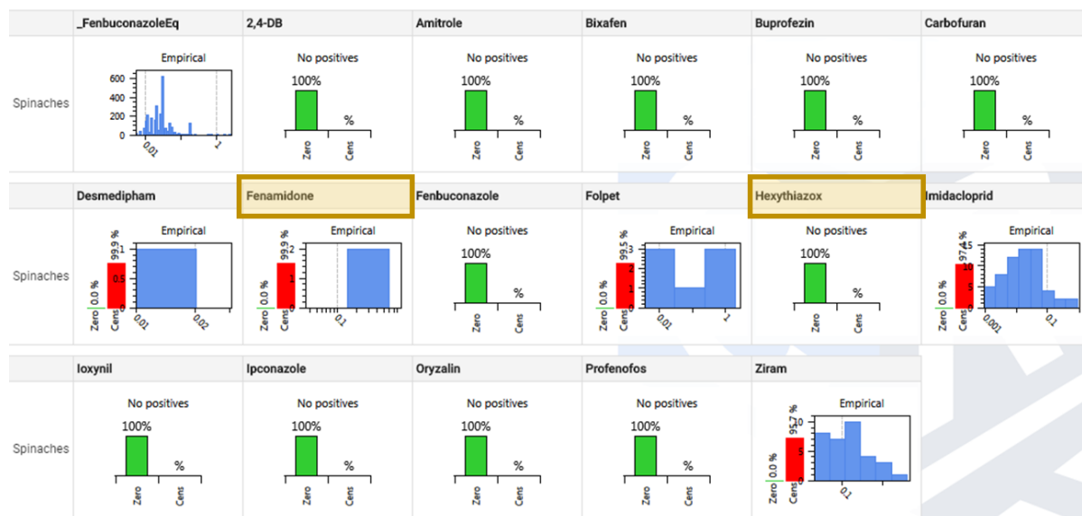
Figure 3.14: Tier 1: Non-detects are not replaced. For Fenamidine and Hexythiazox (brown boxes) authorized use is assumed.
