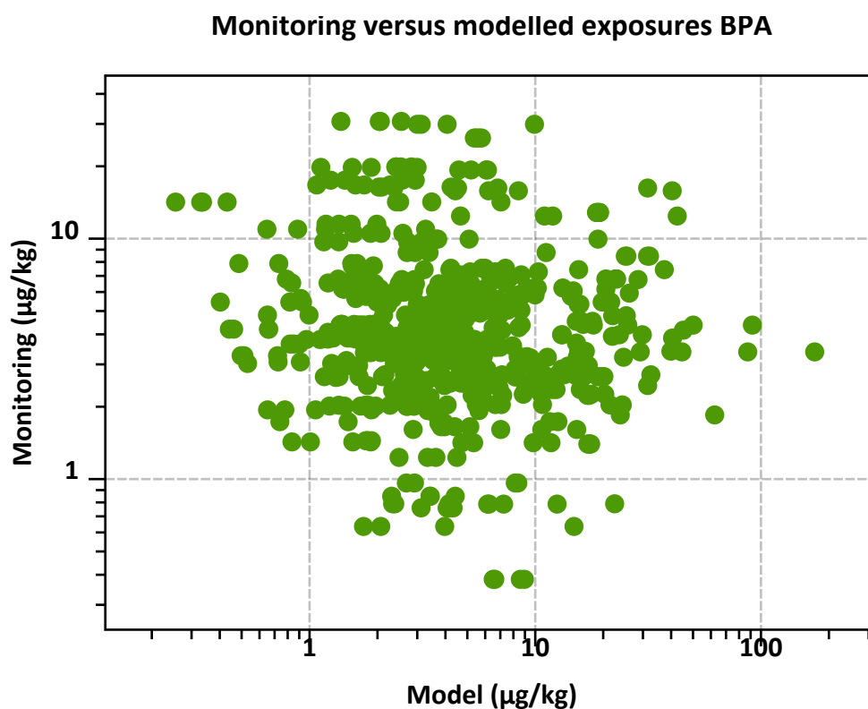
Figure 3.45: Measured exposures from monitoring versus modelled exposures
