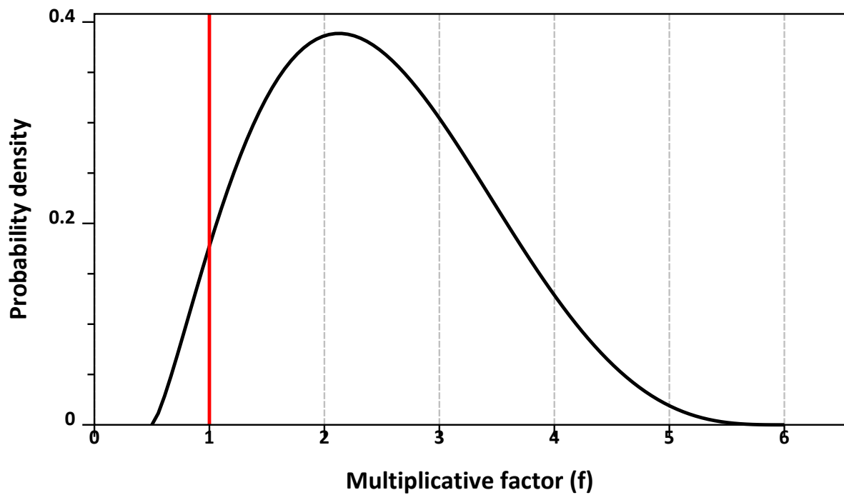
Figure 3.57: Scaled beta ( a=2.37 , b=4.26 , lowerbound=0.5, upperbound=6), table 7, [EFSA (2020a)].
