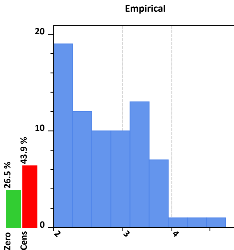
Figure 3.9: Empirical distribution
