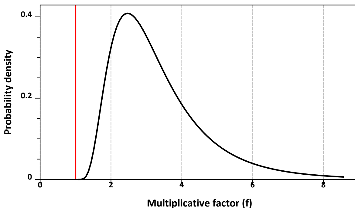
Figure 3.55: Scaled lognormal ( \mu = 0.705 , s = 0.566 , offset=1), table 8, [EFSA (2020b)].
