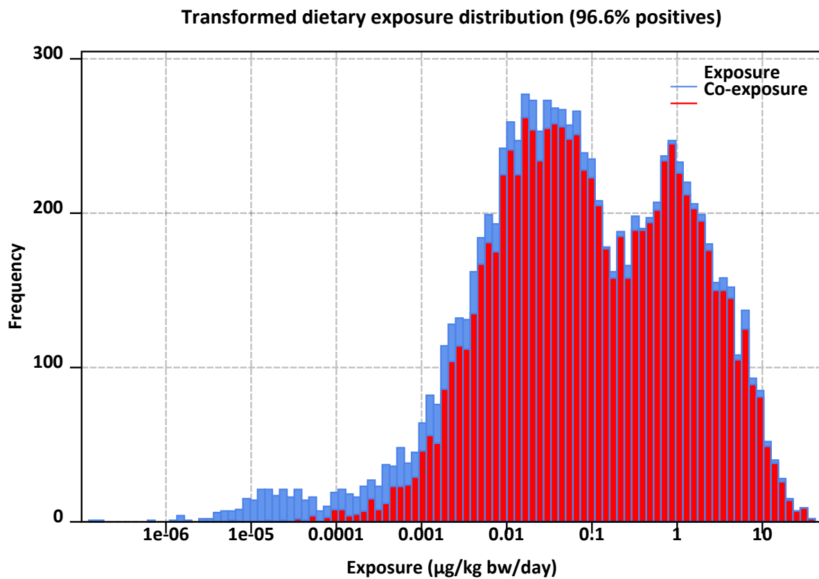
Figure 3.37: Example of co-exposure distribution (from >1 substance per individual-day, red) super-imposed on the total exposure distribution (blue).
