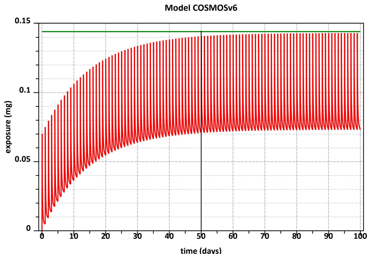
Figure 3.31: Time course of the internal substance amount when applying the same single dose on each day. The acute internal concentration is derived as the peak substance amount (the green line in the figure) divided by the compartment weight. The vertical line at 50 indicates the selected end of an assumed non-stationary period, defining a burn-in period that is to be ignored for computing the peak substance amount.
