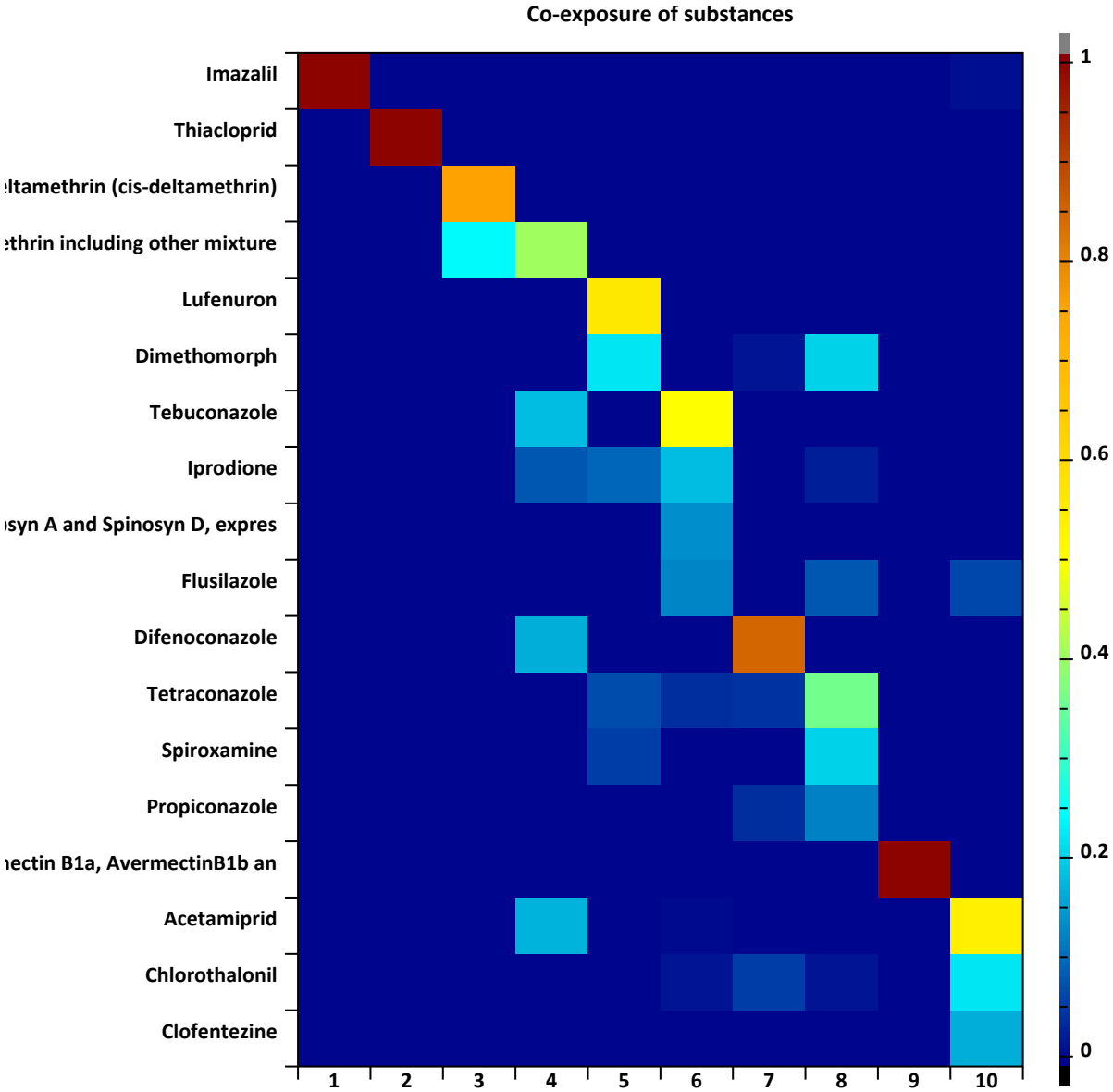
Figure 3.41: Heatmap for a solutions with 10 mixtures. The sparsity is set to 0.4 (sparse). Mixtures contain less substances compared to Figure 3.40 .
