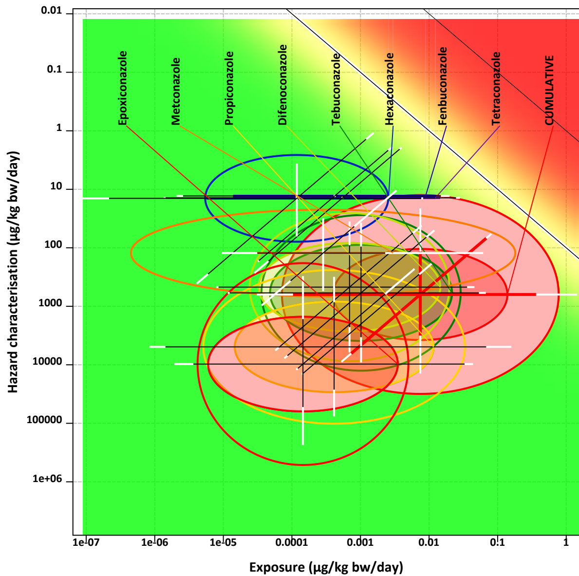
Figure 3.54: Hazard vs. exposure plot for multiple substances. 95% bivariate confidence areas for target hazard dose distribution and exposure distribution. Inner ellipses express variability, outer ellipses uncertainty.
