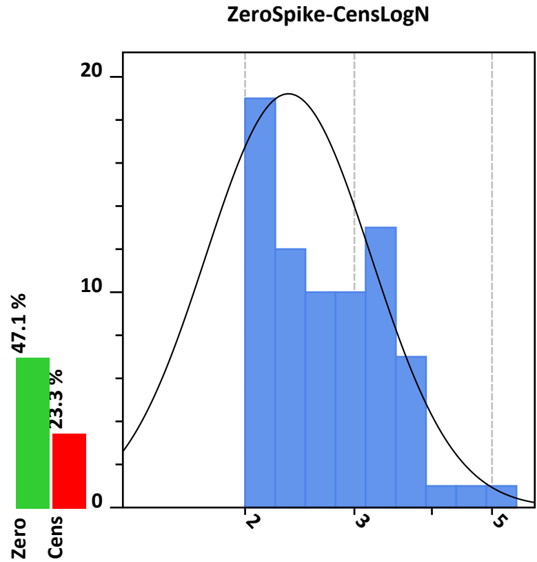
Figure 3.13: Zero Spike Censored Lognormal distribution
