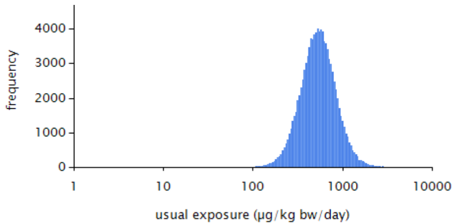
Figure 3.27: Model-assisted estimated usual exposure distributions (excluding the zero exposures).
