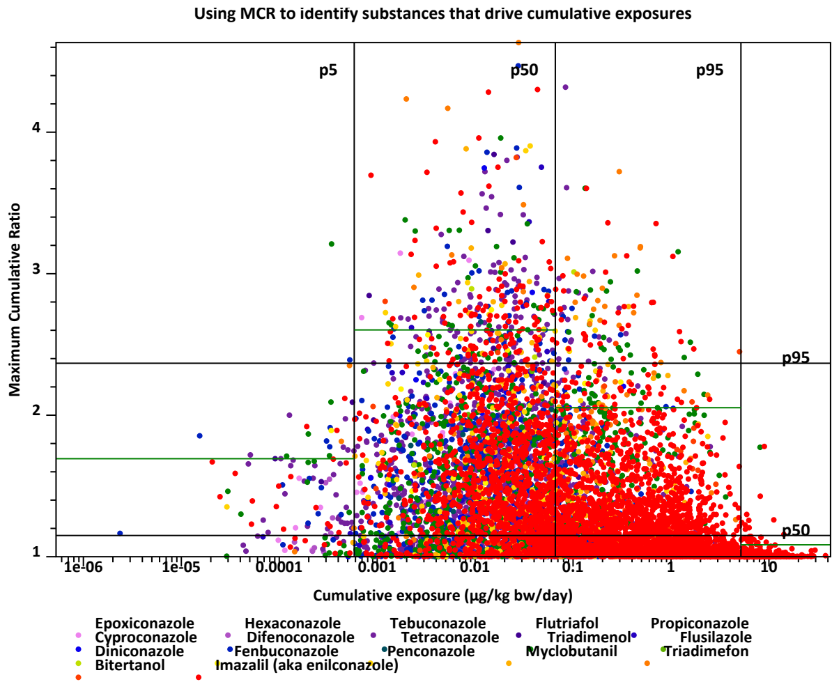
Figure 2.27: Maximum Cumulative Ratios vs total exposure
