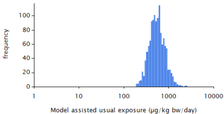
Figure 2.22: Model-based estimated usual exposure distributions (excluding the zero exposures).
