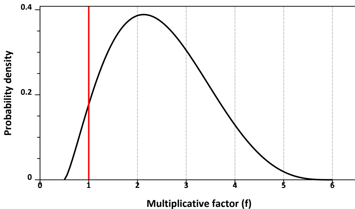
Figure 2.49: Scaled beta ( a=2.37 , b=4.26 , lowerbound=0.5, upperbound=6), table 7, EFSA 2020 [[EFSA, 2020a]].
