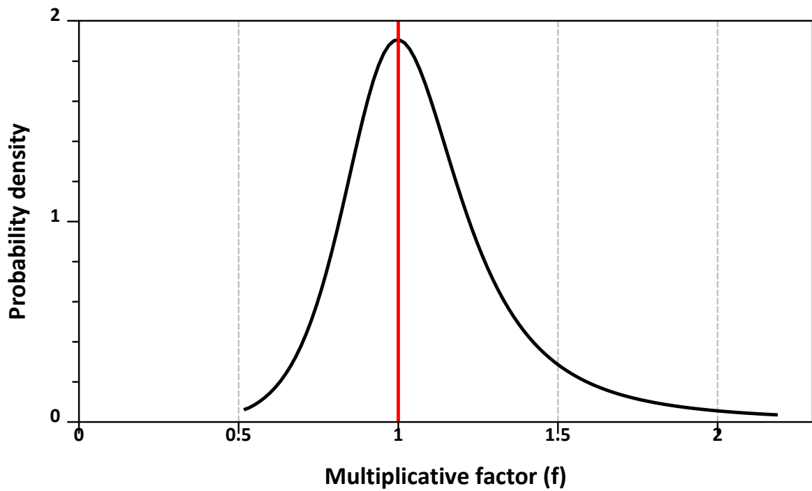
Figure 2.48: Scaled logstudents t ( \mu = -0.593 , s = 0.367 , \nu = 3 , offset=0.5), table 9, EFSA 2020 [[EFSA, 2020b]].
