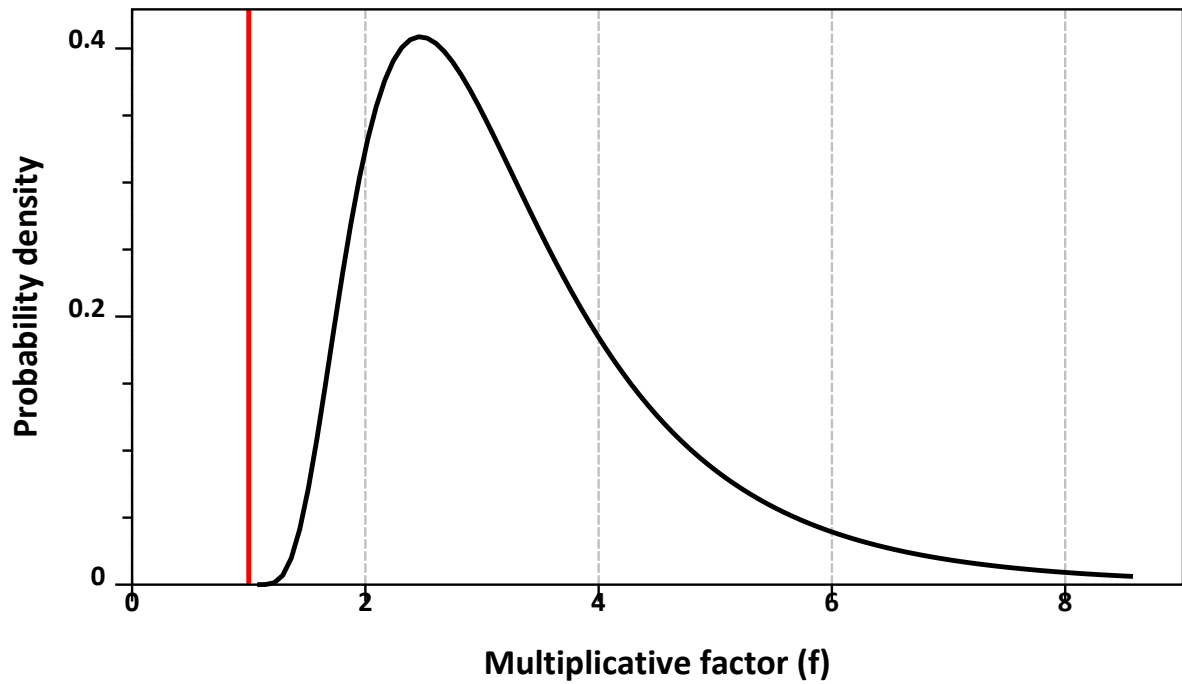
Figure 2.47: Scaled lognormal ( \mu = 0.705 , s = 0.566 , offset=1), table 8, EFSA 2020 [[EFSA, 2020b]].
