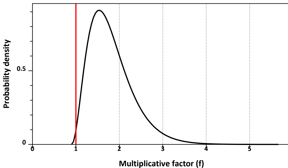
Figure 2.50: Scaled gamma ( a=3.26 , b=3.56 , offset=0.9), table 6, EFSA 2020 [[EFSA, 2020a]].
