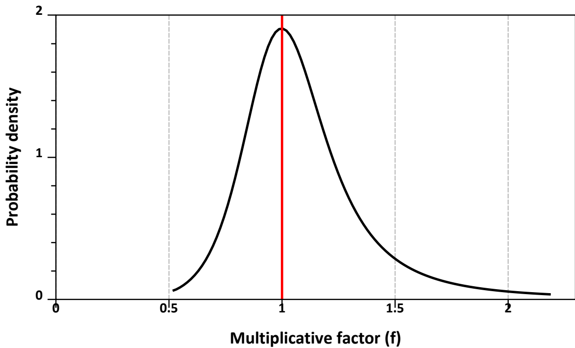
Figure 2.48: Scaled logstudents t ( \mu = -0.593 , s = 0.367 , \nu = 3 , \text{offset} = 0.5 ), table 9, EFSA 2020 [EFSA, 2020b].
