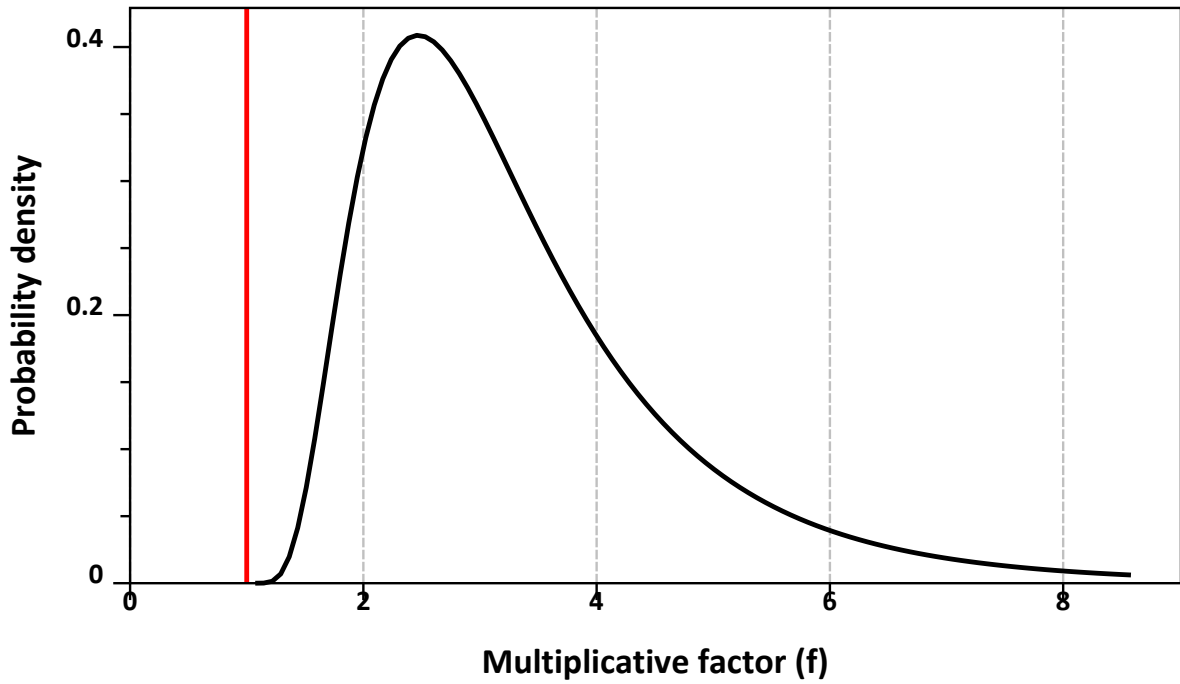
Figure 2.47: Scaled lognormal ( \mu = 0.705 , s = 0.566 , \text{offset} = 1 ), table 8, EFSA 2020 [EFSA, 2020b].
