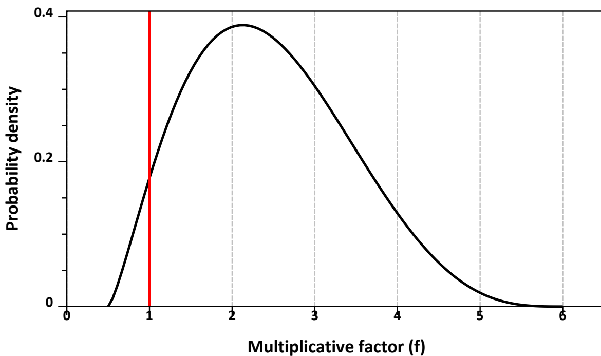
Figure 2.48: Scaled beta ( a = 2.37 , b = 4.26 , \text{lowerbound} = 0.5 , \text{upperbound} = 6 ), table 7, EFSA 2020 [EFSA, 2020a].
