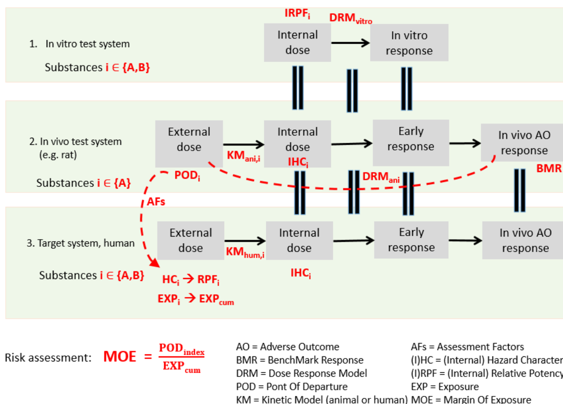
Figure 2.35: Conceptual model IVIVE.
