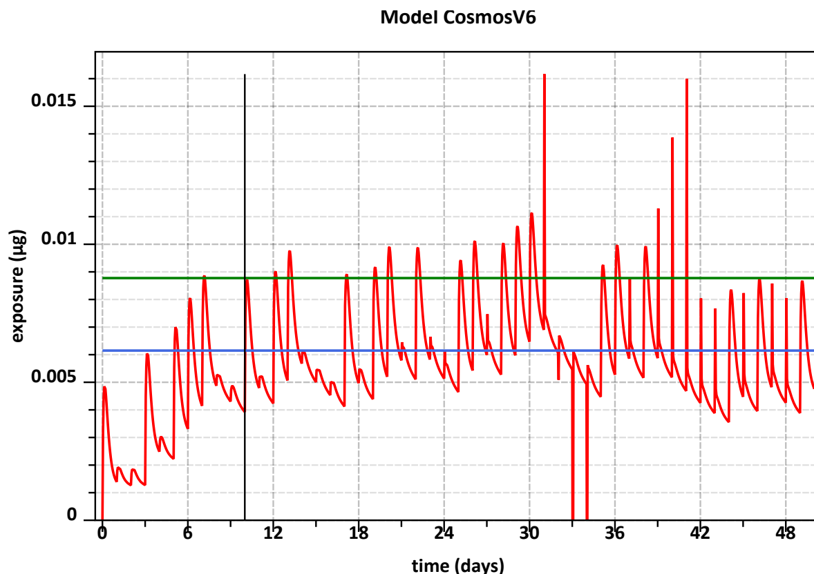
Figure 2.37: Time course of exposure ( \mu\text{g} ) for Clothianidin in the liver (COSMOS version 6).
