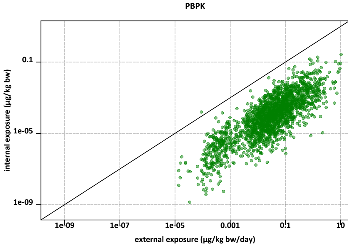
Figure 2.38: Internal versus external exposure for Clothianidin in the liver (COSMOS version 6).
