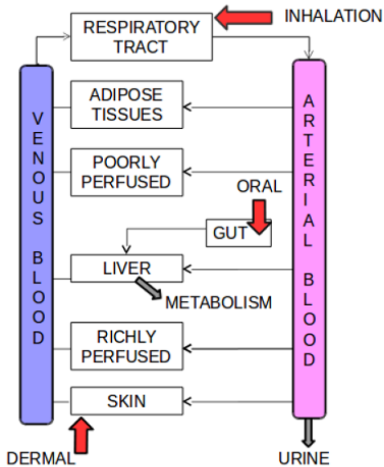
Figure 2.36: Schematic representation of the 'COSMOS' PBPK model.
