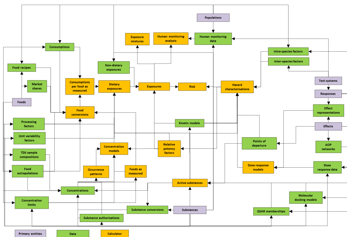
Figure 2.1: Diagram of the modular design of MCRA.
