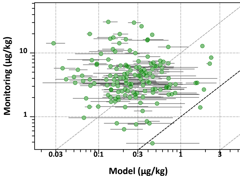
Figure 3.68: Monitoring versus modelled concentrations for bisphenol BPA
