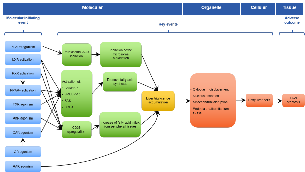
Figure 3.74: AOP network
