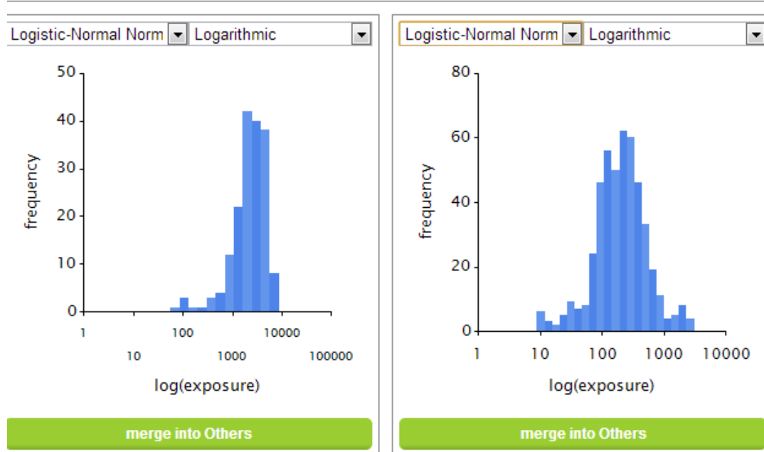
Figure 3.34: Result of a selection into two split-off groups and a rest group. The graph bottom left represents the exposure via a food group containing ‘Sausage, frankfurter’ and ‘Sausage, smoked cooked’. The graph bottom right represents the exposure via a food group containing ‘Sausage, luncheon meat’, Herbs, mixed, main brands, not prepared’, ‘Soup, pea’, ‘Ham’, and ‘Bacon’. The top graph represents the exposure via the rest group.
