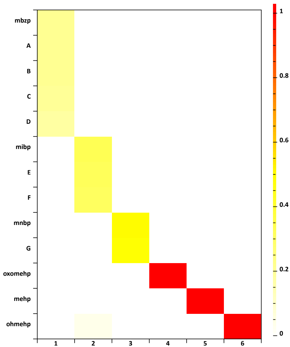
Figure 3.64: SNMU solution with 6 components. Sparsity = 0.8.
