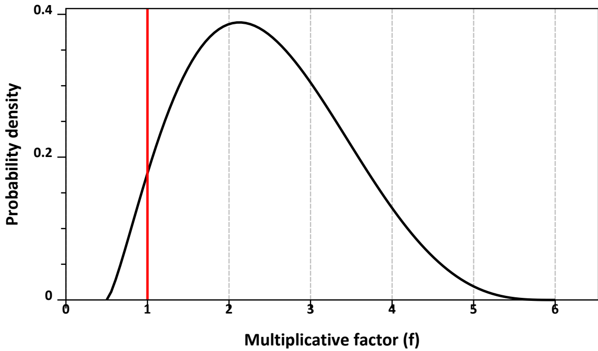
Figure 3.90: Scaled beta ( a=2.37 , b=4.26 , lowerbound=0.5, upperbound=6), table 7, EFSA (2020a).
