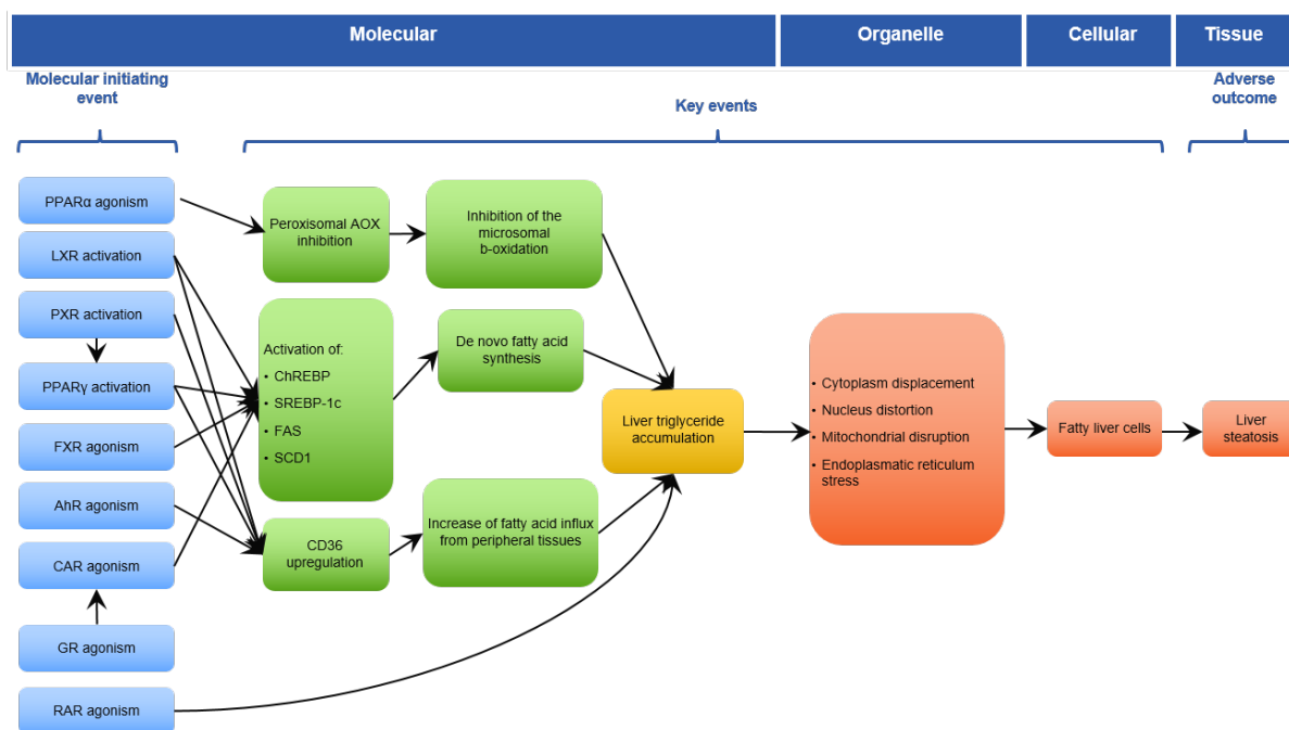
Figure 3.72: AOP network
