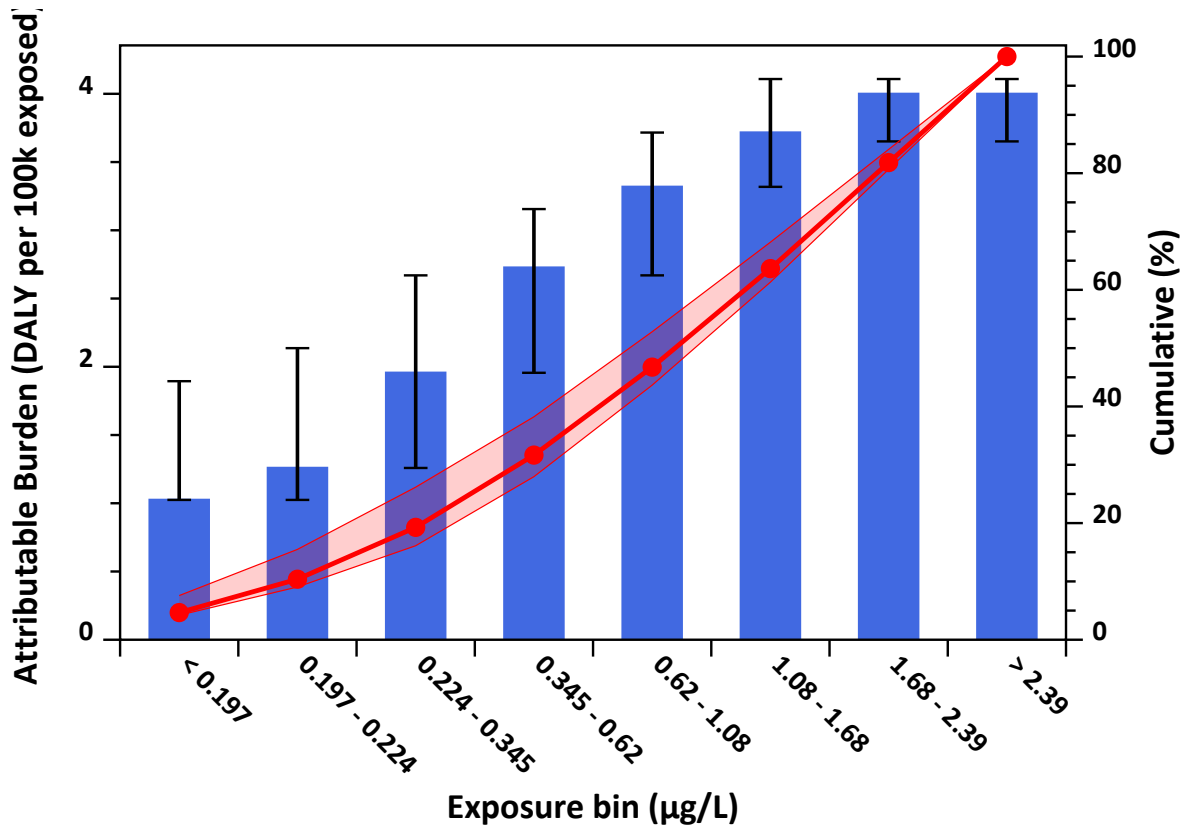
Figure 3.82: EBD per 100,000 individuals & cumulative percentage
