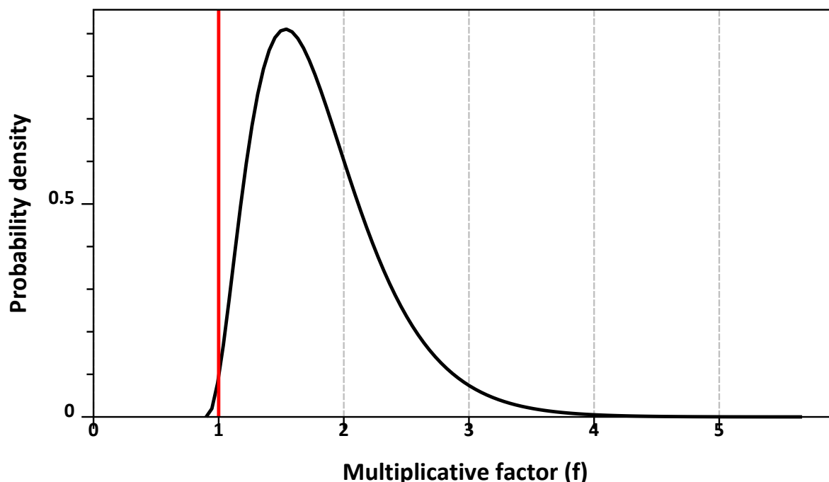
Figure 3.89: Scaled gamma ( a=3.26 , b=3.56 , offset=0.9 ), table 6, EFSA (2020a).
