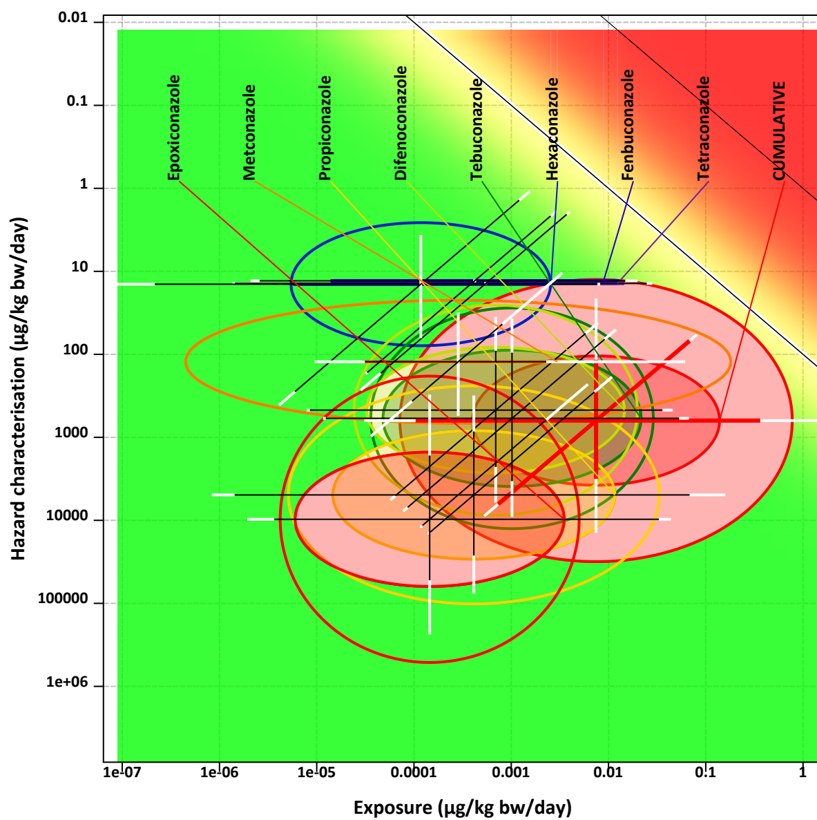
Figure 3.92: Hazard vs. exposure plot for multiple substances. 95% bivariate confidence areas for target hazard dose distribution and exposure distribution. Inner ellipses express variability, outer ellipses uncertainty.
