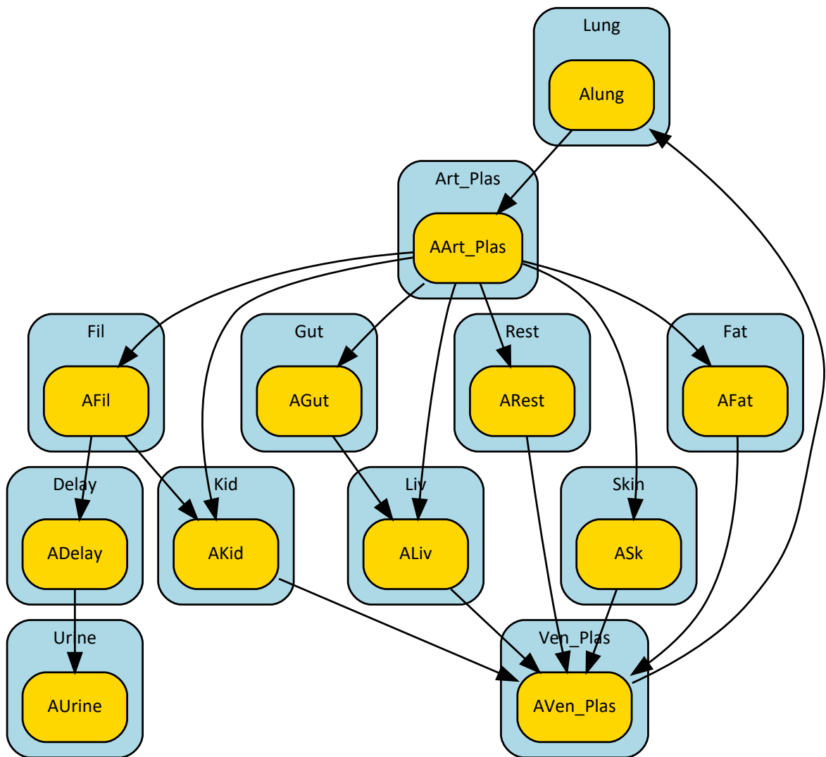
Figure 3.79: Kinetic compartments
