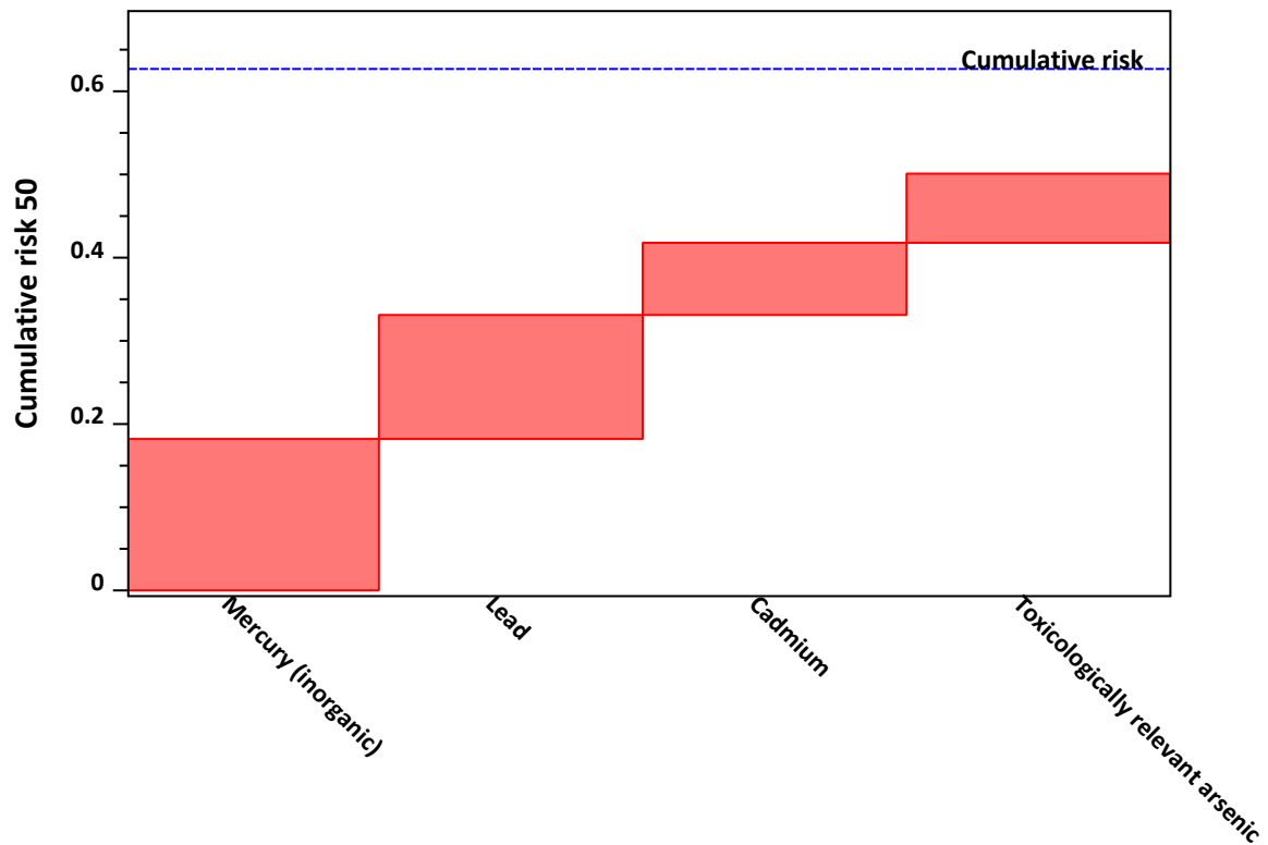
Figure 3.93: Cumulative risk characterisation ratios exposure/hazard (median) in the population (metals).
