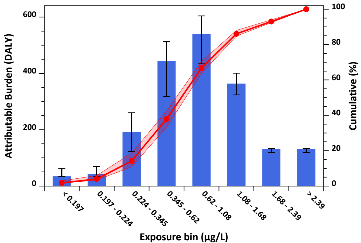
Figure 3.86: Attributable burden &amp; cumulative percentage with ERF defined bins
