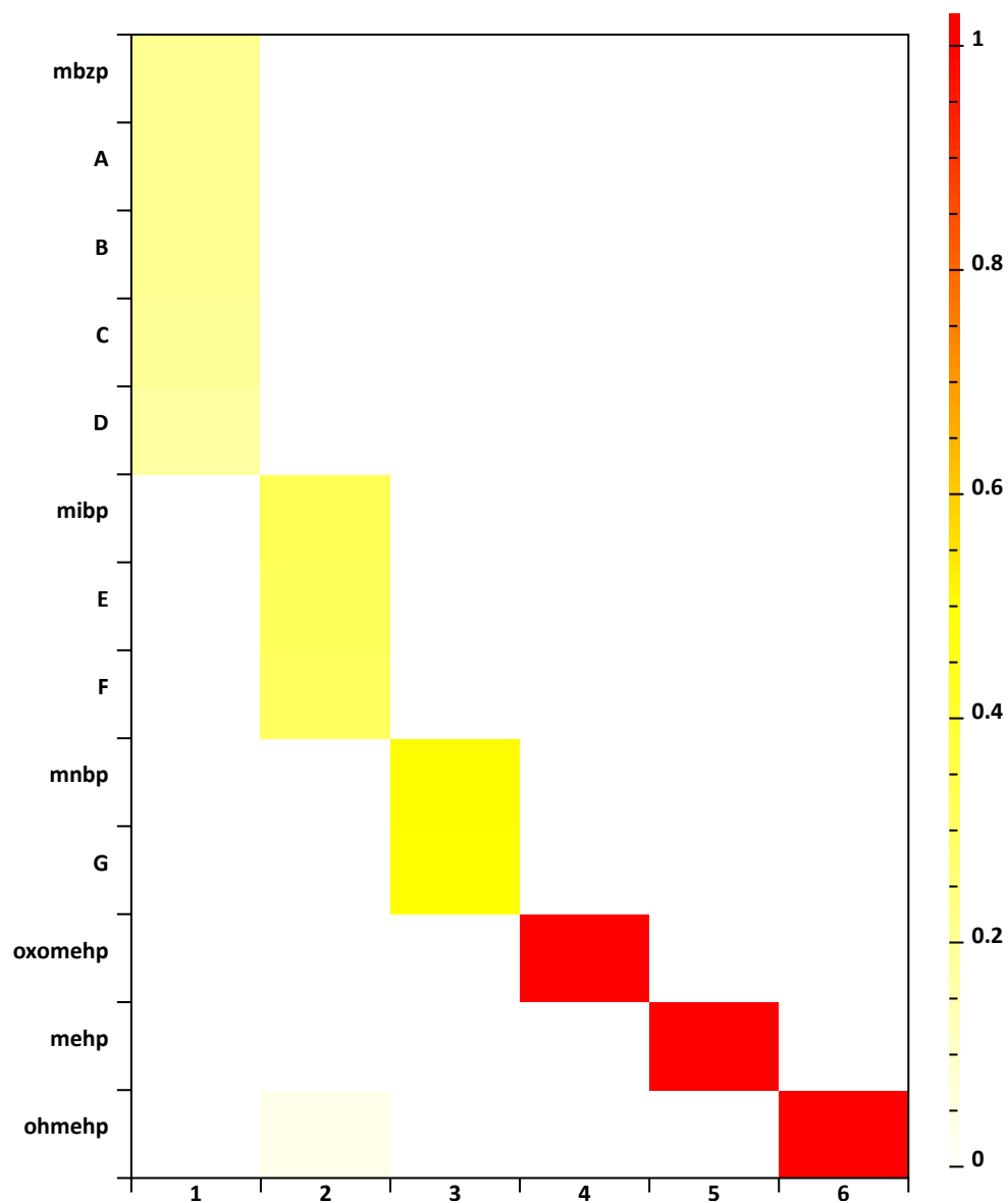
Figure 3.65: SNMU solution with 6 components. Sparsity = 0.8.
