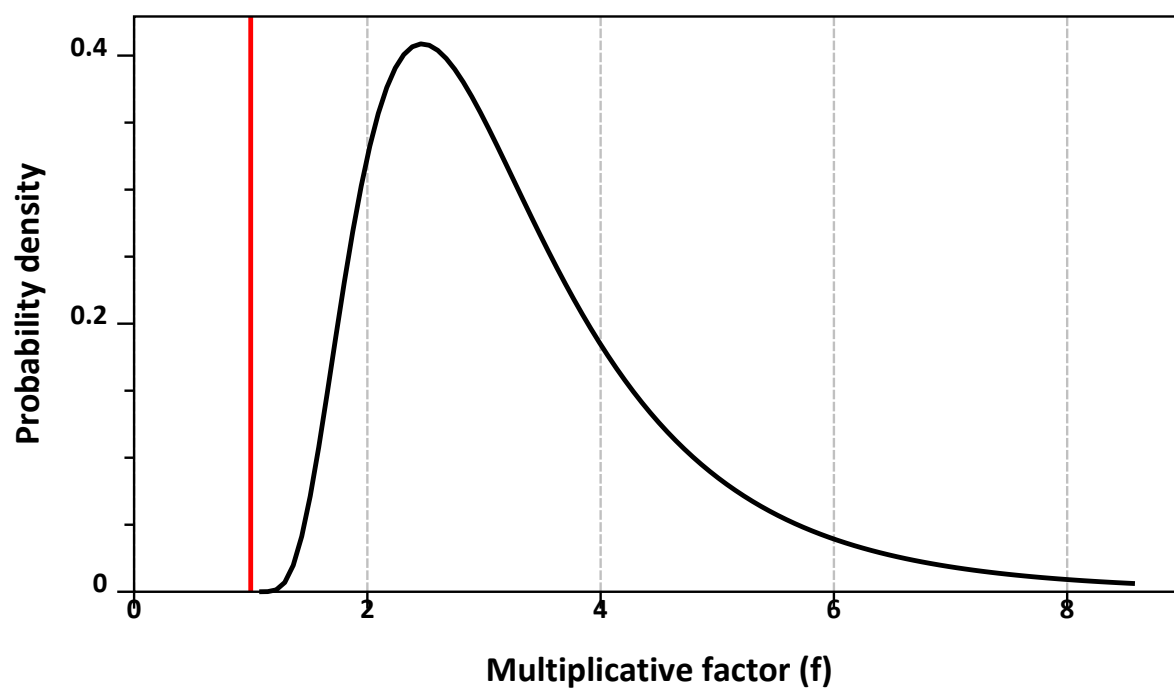
Figure 3.96: Scaled lognormal ( \mu = 0.705 , s = 0.566 , offset=1), table 8, EFSA (2020b) .
