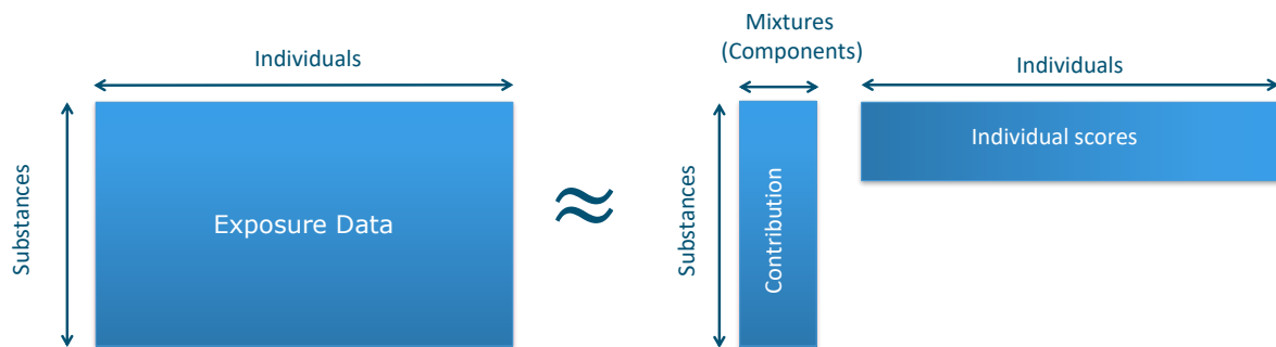
Figure 3.53: SNMU approximation of exposure data after scaling.
