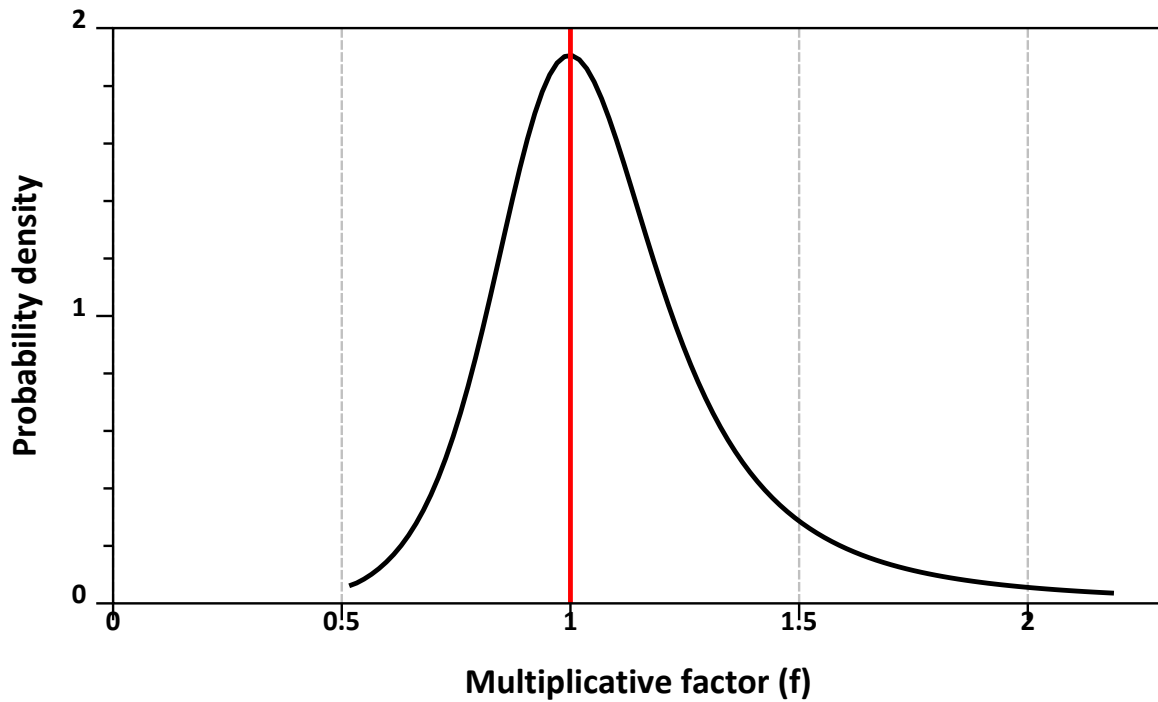
Figure 3.97: Scaled logstudents t ( \mu = -0.593 , s = 0.367 , \nu = 3 , offset=0.5), table 9, EFSA (2020b) .
