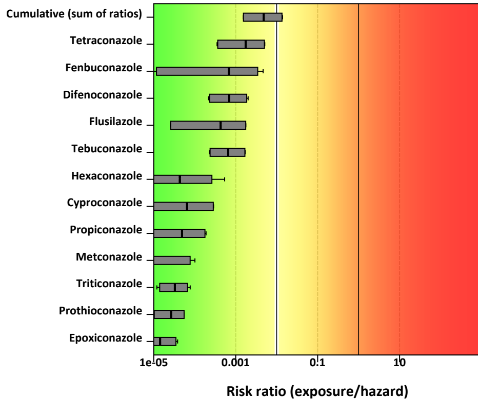
Figure 3.91: Risk characterisation ratio (exposure/hazard) plot for multiple substances (triazoles). The threshold of 0.01 is indicated with the left vertical line, the vertical black line on the right indicates a threshold of 1.
