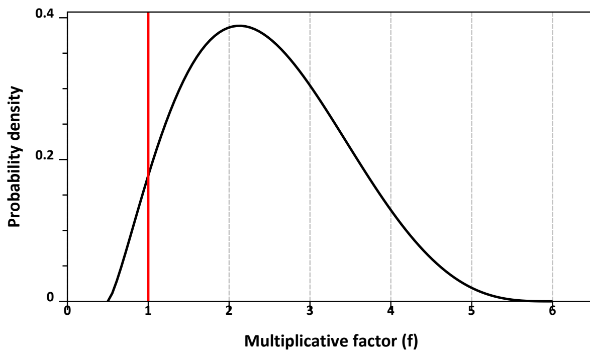
Figure 3.95: Scaled beta ( a=2.37 , b=4.26 , lowerbound=0.5, upperbound=6), table 7, EFSA (2020a) .
