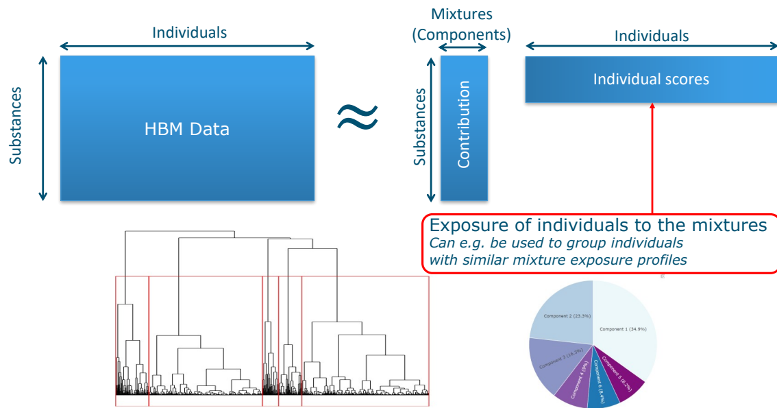
Figure 3.60: SNMU: matrix V , individual scores to components.
