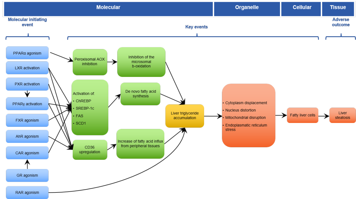
Figure 3.74: AOP network
