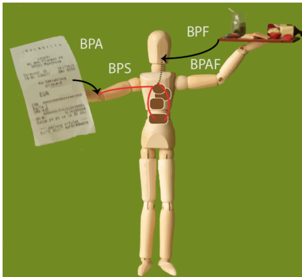
Figure 3.83: Graphical abstract ‘Linking probabilistic exposure and pharmacokinetic modelling to assess the cumulative risk from the bisphenols BPA, BPS, BPF, and BPAF for Europeans.’
