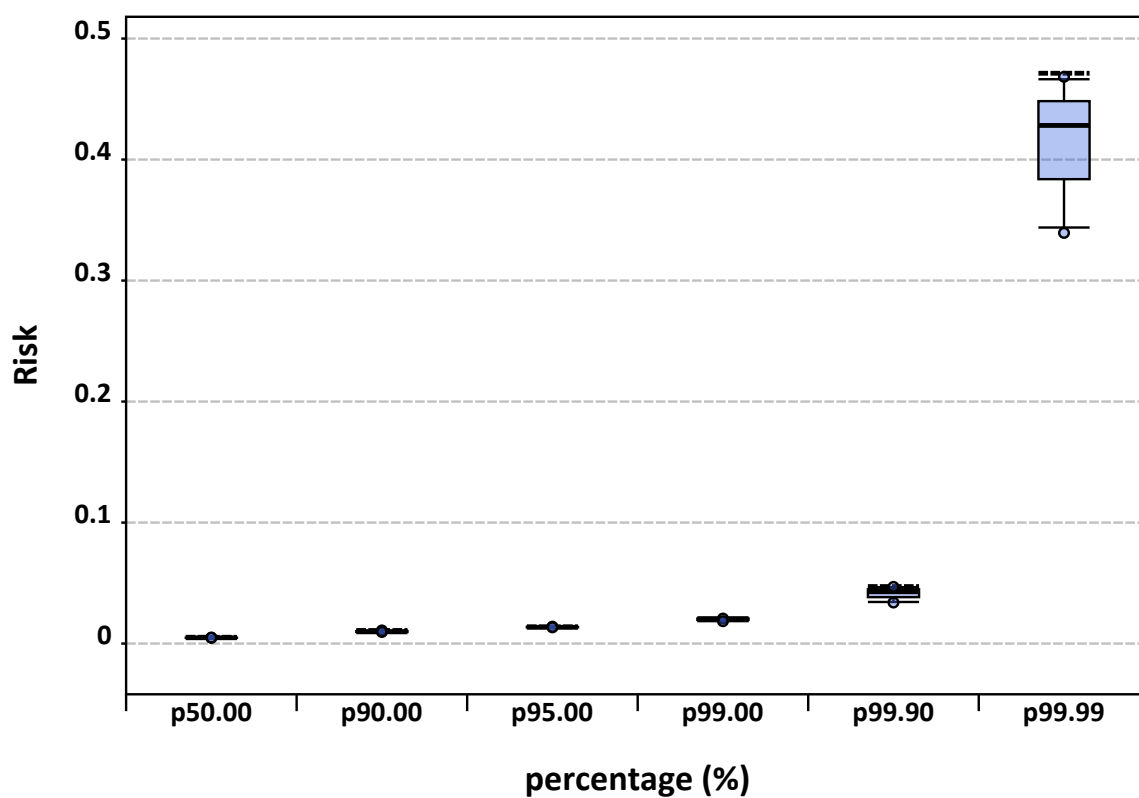
Figure 3.90: Uncertainty of percentiles. The boxplots for uncertainty show the p25 and p75 as edges of the box, and p2.5 and p97.5 as edges of the whiskers. The reference (nominal) value is indicated with the dashed black line, the median with the solid black line within the box. Outliers are displayed as dots outside the whiskers. Risk is specified as the characterisation ratio (exposure/hazard) (triazoles).
