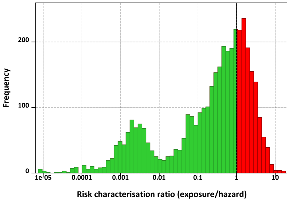
Figure 3.77: Risk characterisation ratio (exposure/hazard) based on BMDL, POCE = 32\% .
