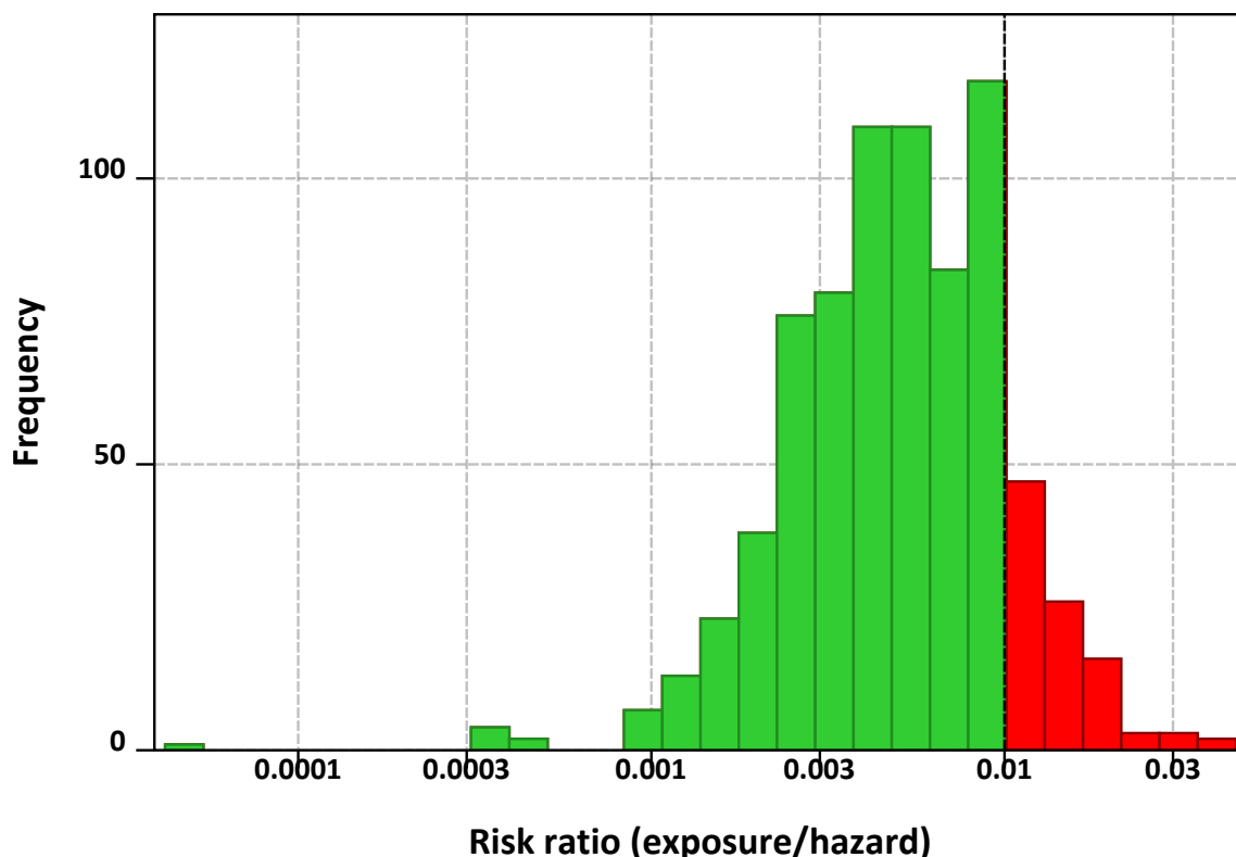
Figure 3.89: Risk characterisation ratio (exposure/hazard) total distribution (triazoles) with a threshold of 0.01.
