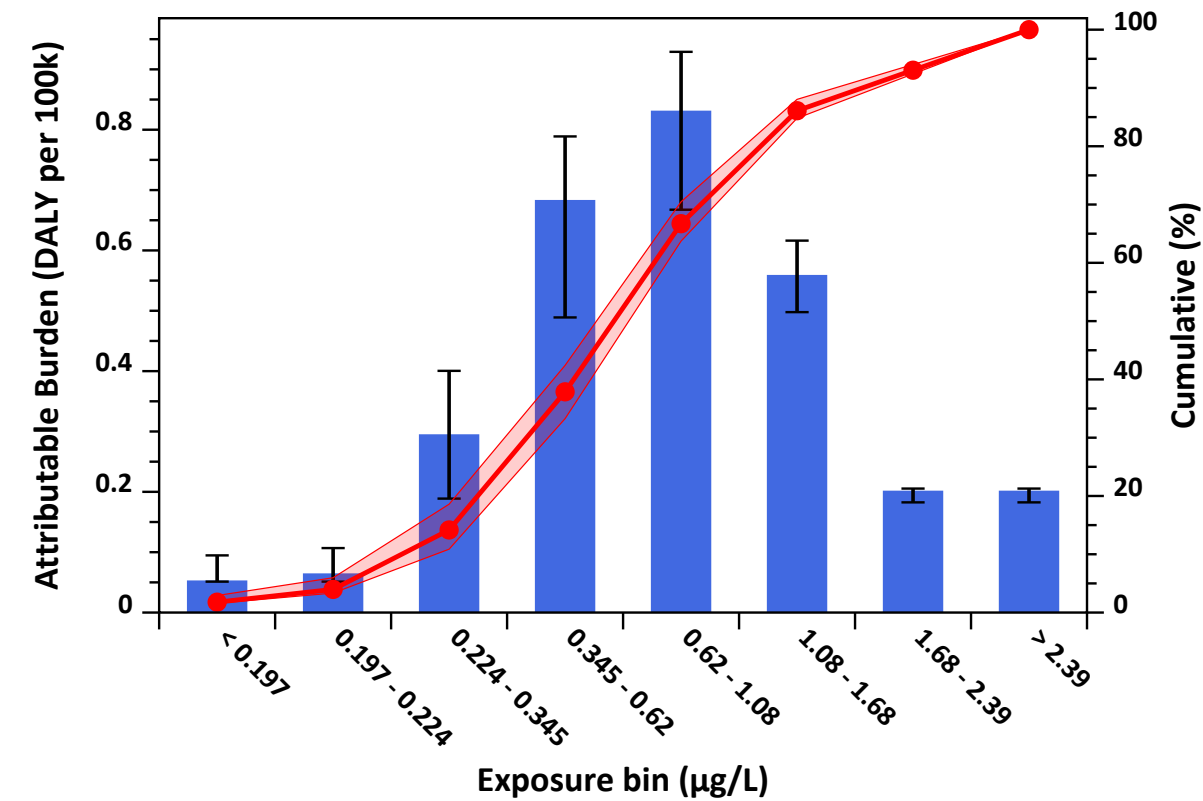
Figure 3.87: EBD per 100,000 individuals & cumulative percentage with ERF defined bins
