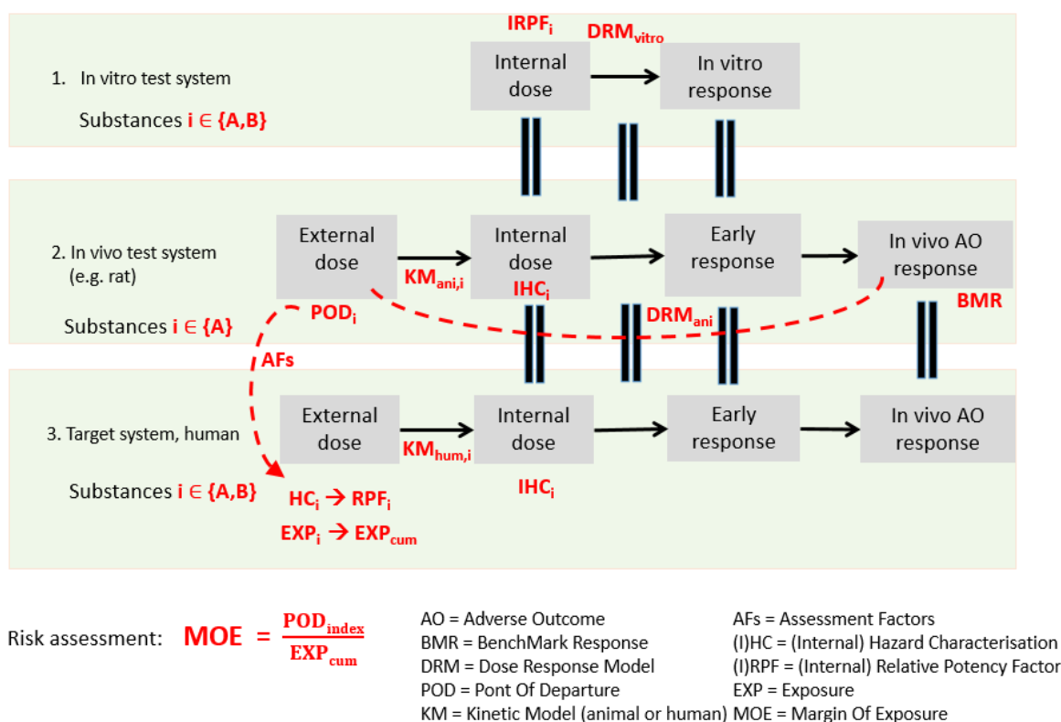
Figure 3.78: Conceptual model IVIVE.
