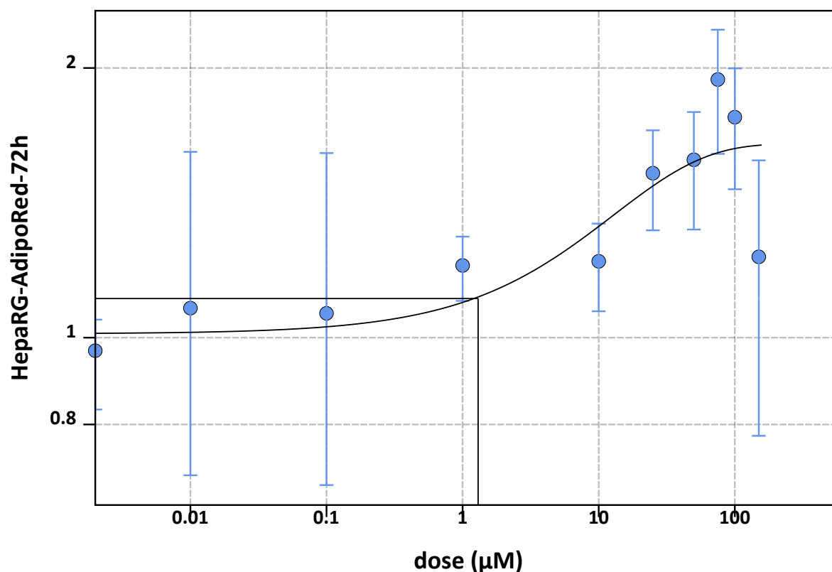
Figure 3.75: Dose response model: HepaRG Adipo72 72h.
