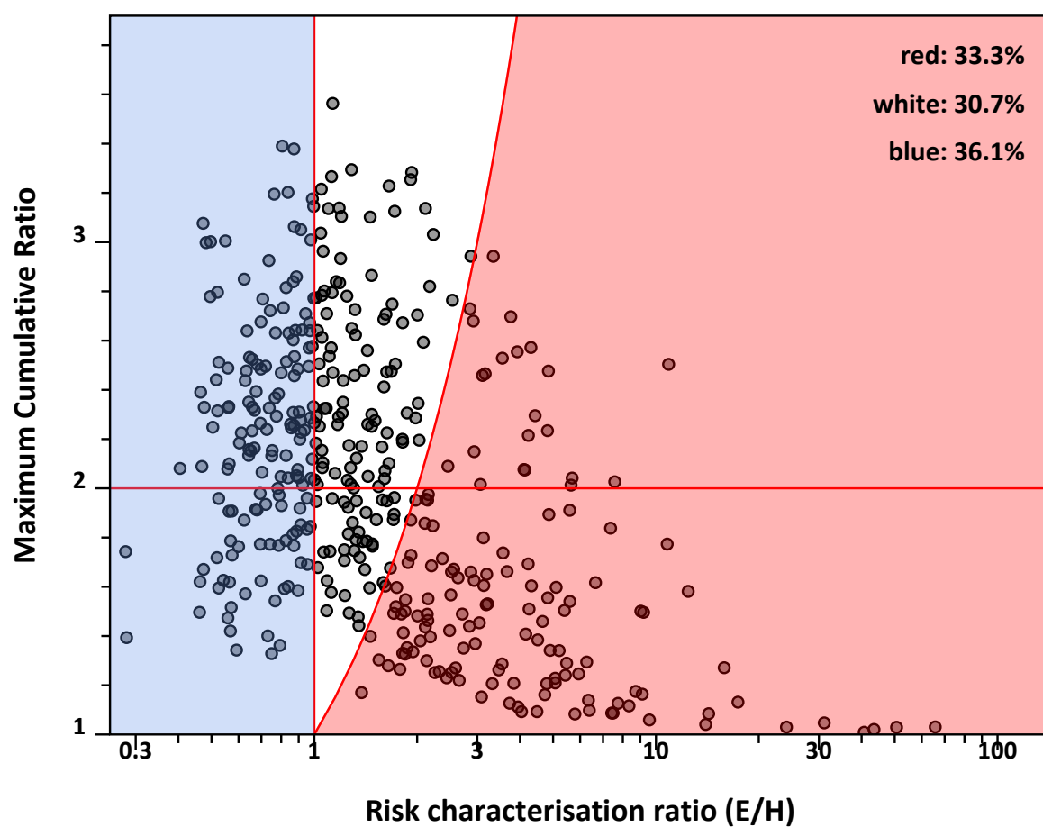
Figure 3.50: Using MCR to identify substances that drive cumulative risk, scatter distributions (total).
