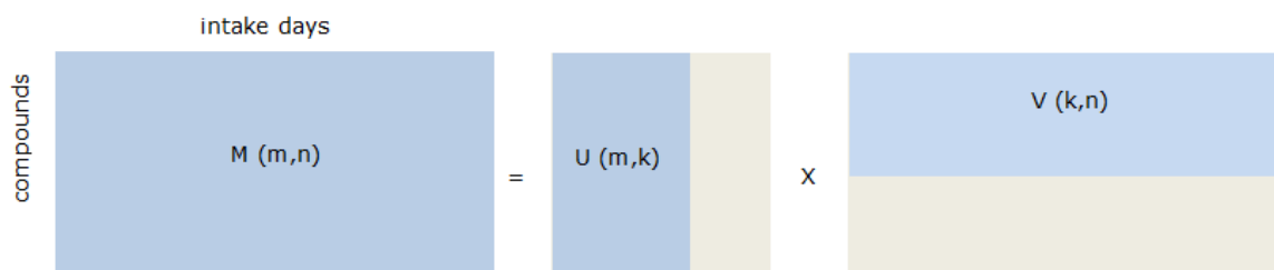
Figure 3.52: NMF approximation of exposure data
