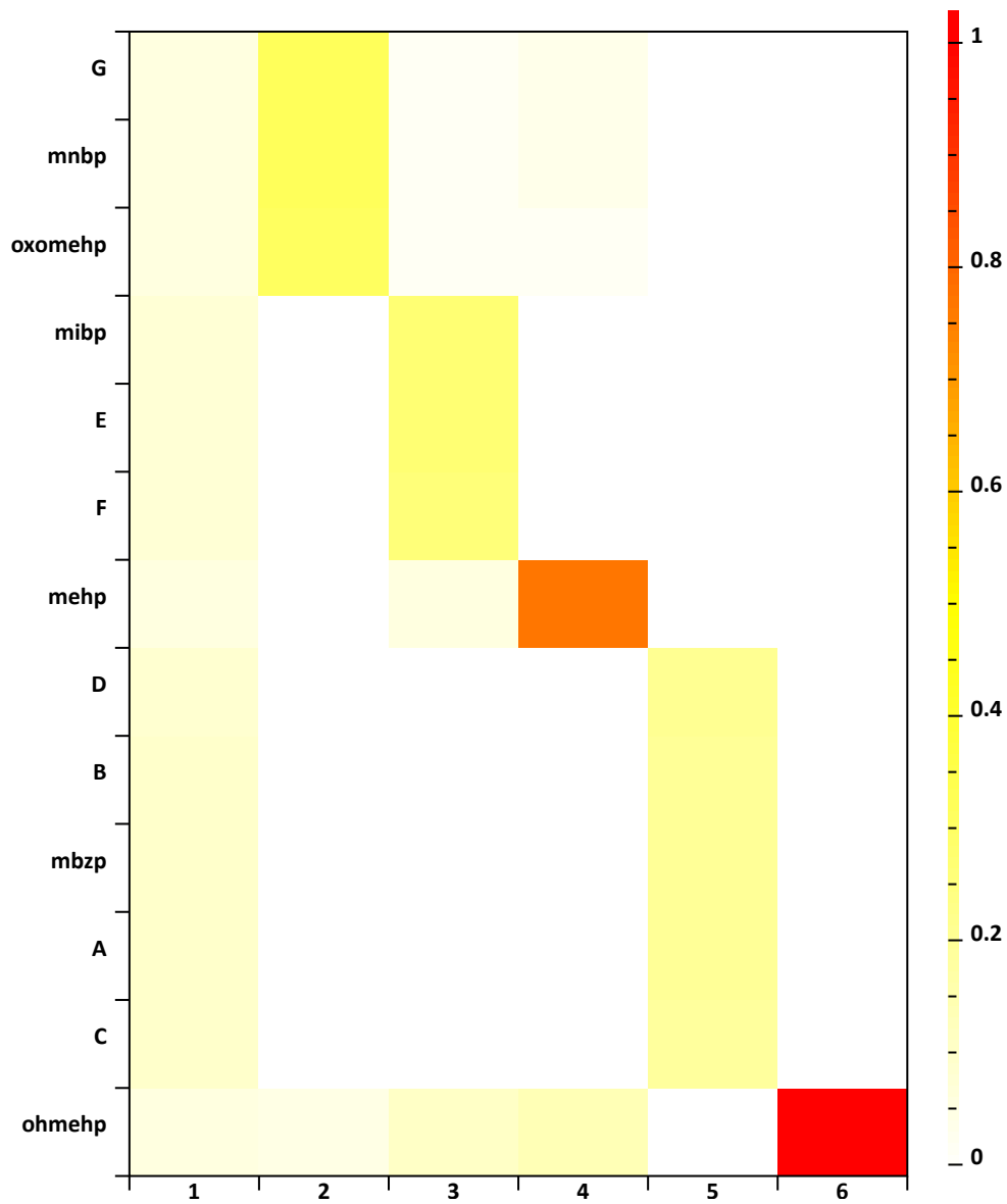
Figure 3.56: Co-exposure of substances. Heatmap for a solution with 6 components. The sparsity = 0.1. Each component, especially the first, contains many substances (see also Figure 3.57 ).
