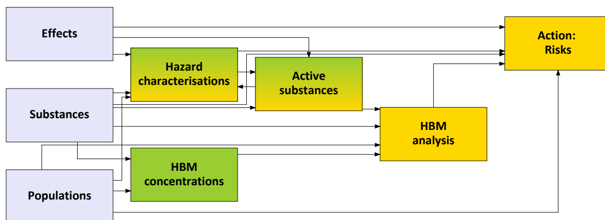
Figure 3.84: Risks module.
