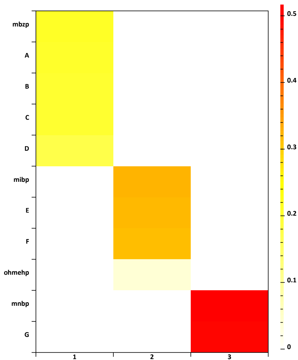
Figure 3.59: Heatmap for solution with 3 components. The first 3 components in Figure 3.59 and Figure 3.57 contain the same substances.
