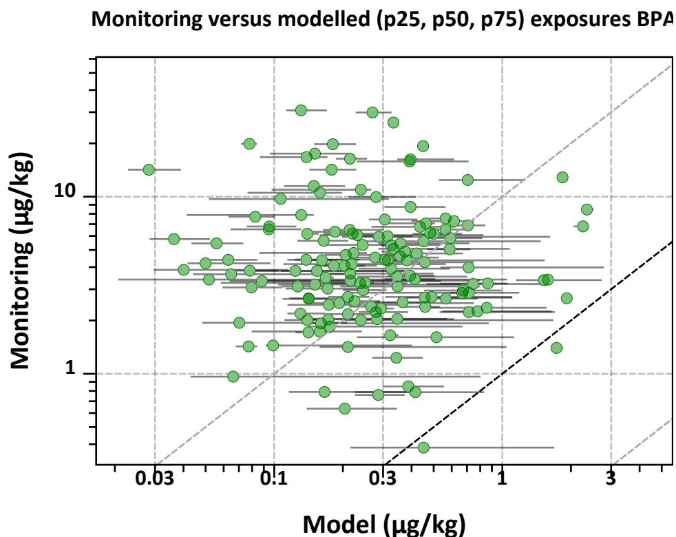
Figure 3.67: Monitoring versus modelled concentrations for bisphenol BPA
