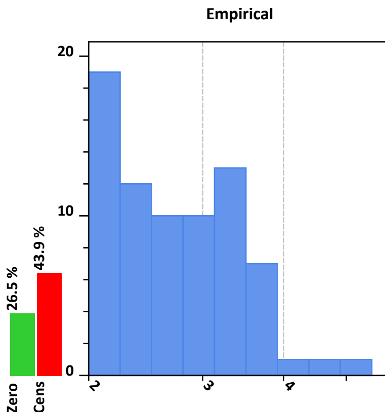
Figure 3.16: Empirical distribution
