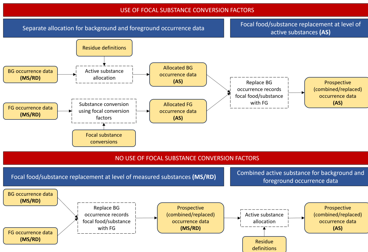
Figure 3.27: Active substance allocation of the background and foreground concentration data with and without the use of deterministic substance conversion factors.
