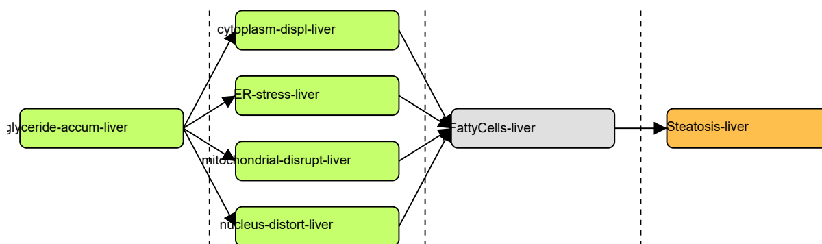
Figure 3.71: AOP network liver steatosis
