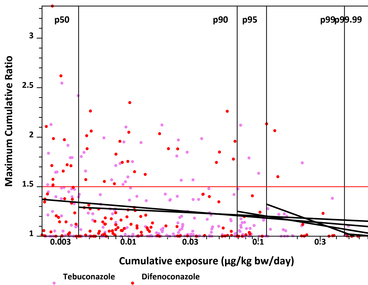
Figure 3.45: Using MCR to identify substances that drive cumulative exposures, scatter distributions (upper tail 37%).
