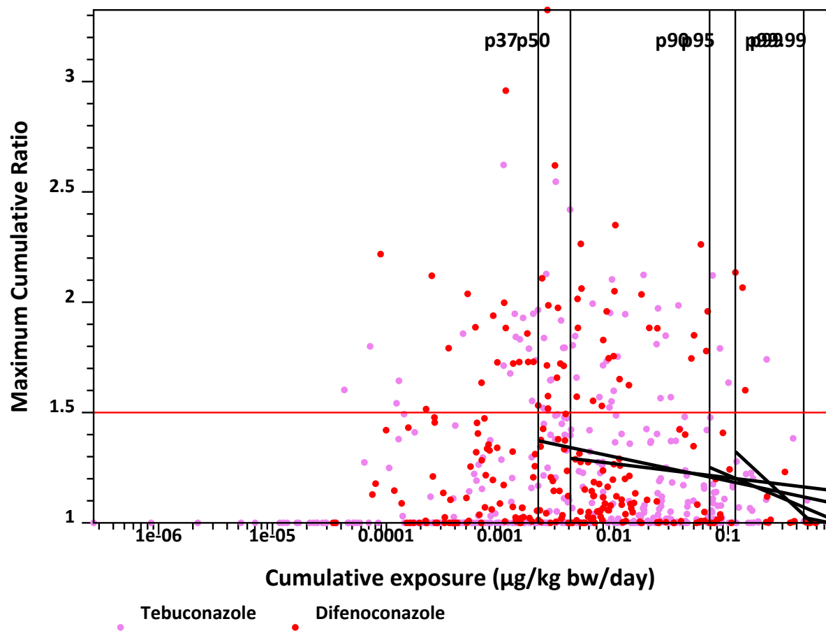
Figure 3.44: Using MCR to identify substances that drive cumulative exposures, scatter distributions (total).
