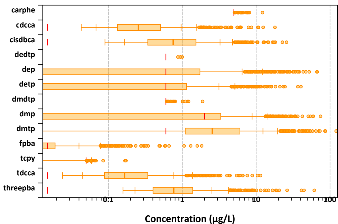
Figure 3.66: Boxplots for all of HBM substance concentration measurements of 13 pesticides. Lower whiskers indicate the p5 and p10 percentiles, upper whiskers the p90 and p95. The edges of the box indicate the p25 and p75 percentiles with the median in the centre of the box. LORs are displayed by a vertical red bar and outliers outside range ( Q1 - 3 * IQR , Q3 + 3 * IQR ).
