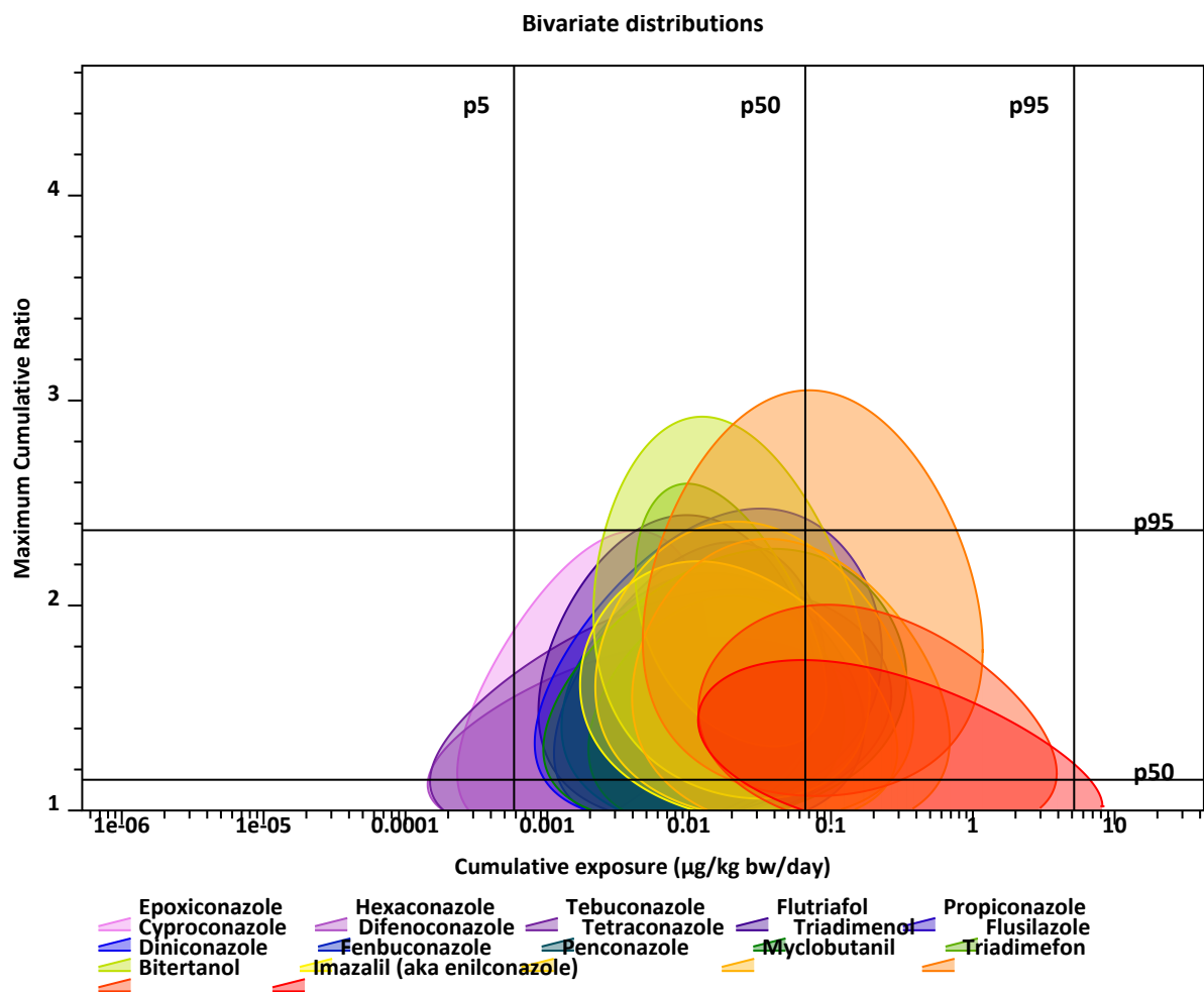
Figure 3.43: Bivariate distributions MCR vs total exposure
