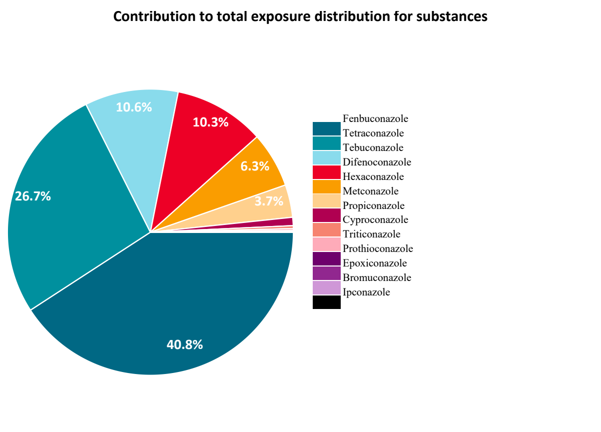
Figure 3.31: Example MCRA dietary exposure contributions substances
