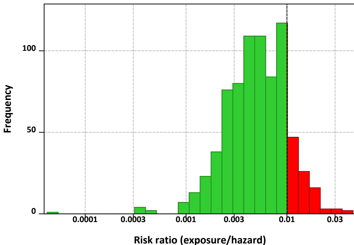
Figure 3.77: Risk characterisation ratio (exposure/hazard) total distribution (triazoles).
