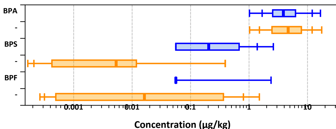
Figure 3.62: Boxplots for monitoring and modelled concentrations for bisphenols BPA, BPS and BPF. Lower whiskers indicate the p5 and p10 percentiles, upper whiskers the p90 and p95. The edges of the box indicate the p25 and p75 percentiles with the median in the centre of the box.
