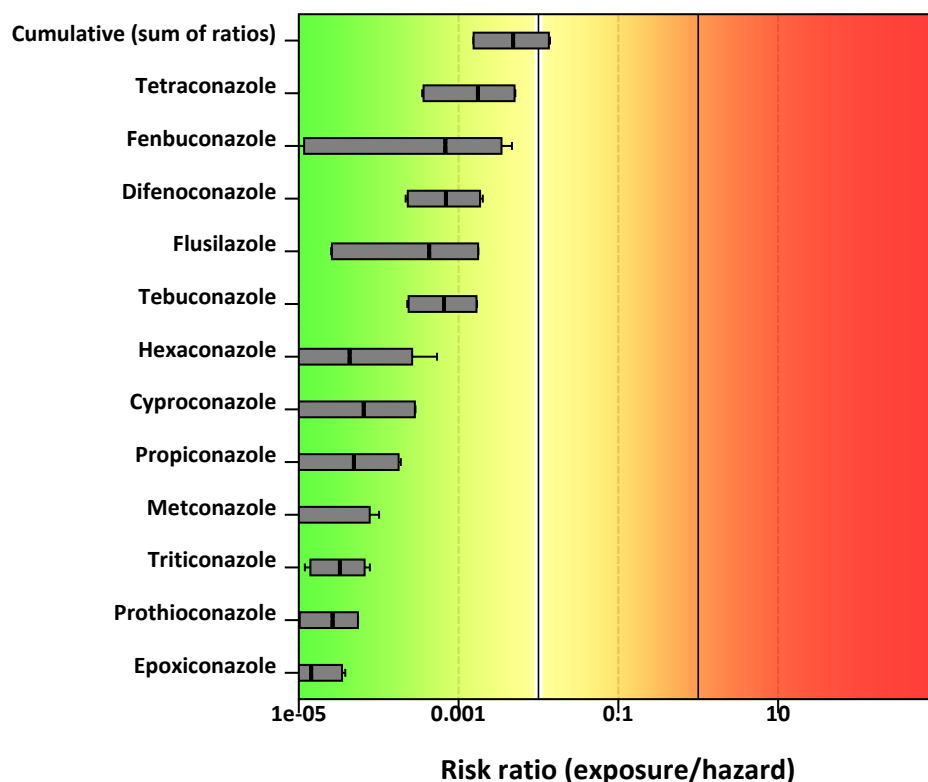
Figure 3.79: Risk characterisation ratio (exposure/hazard) plot for multiple substances (triazoles). The threshold (0.01) is indicated with the left vertical line, the vertical black line on the right indicates threshold value = 1.
