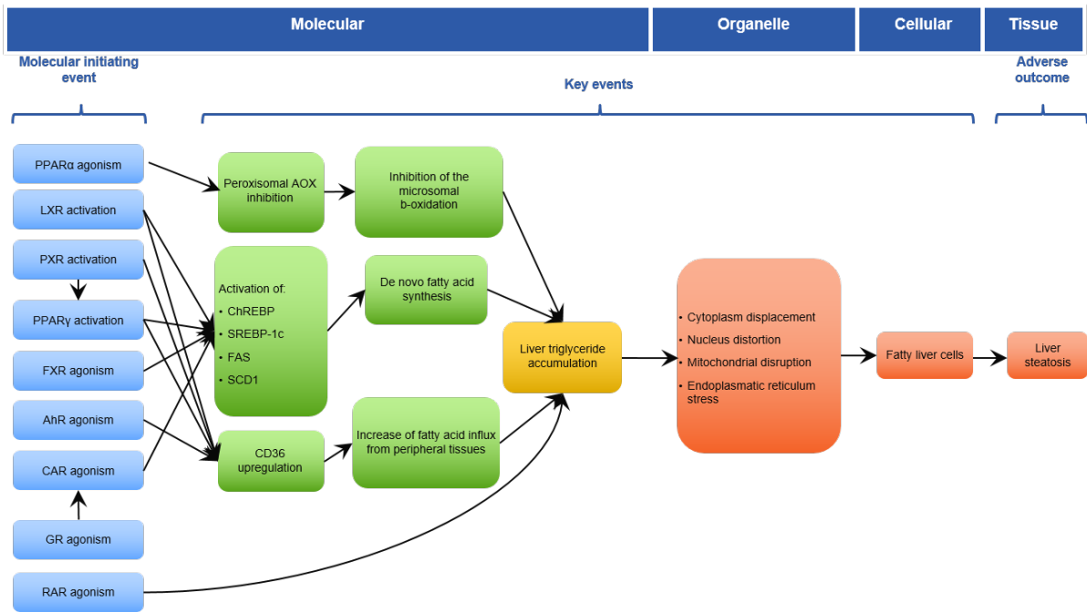
Figure 3.68: AOP network
