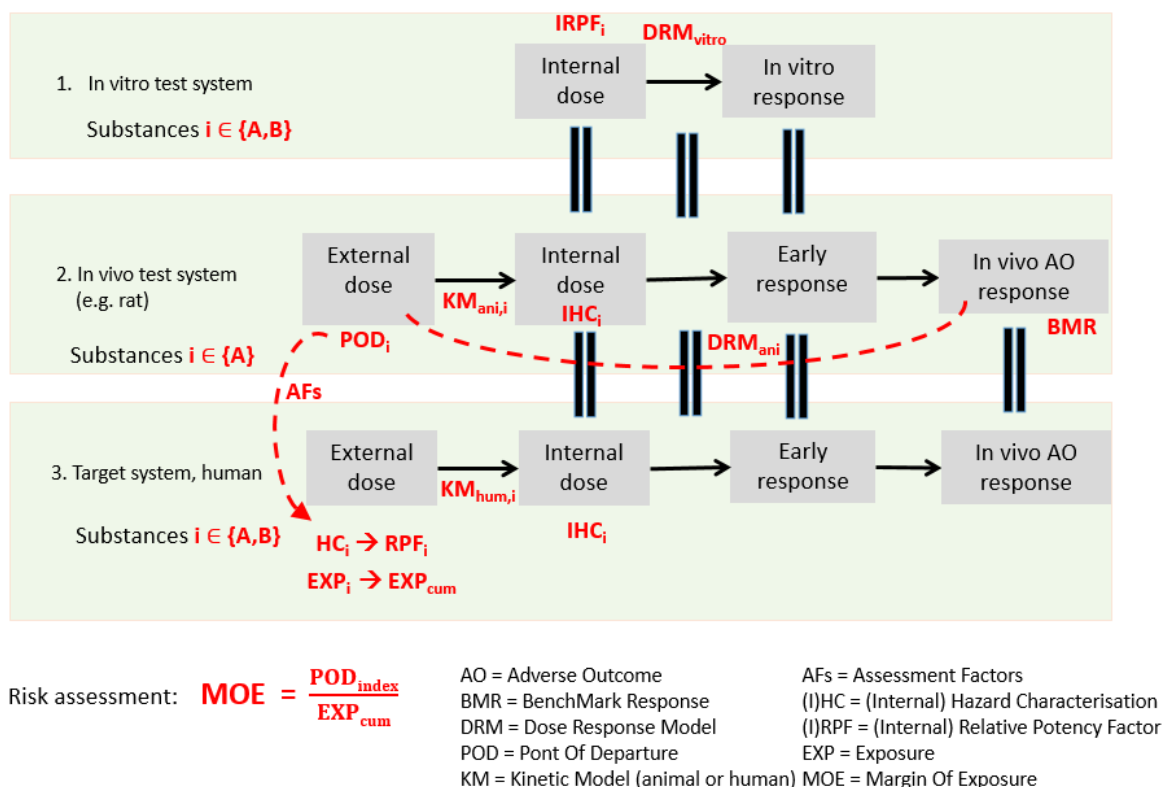
Figure 3.72: Conceptual model IVIVE .
