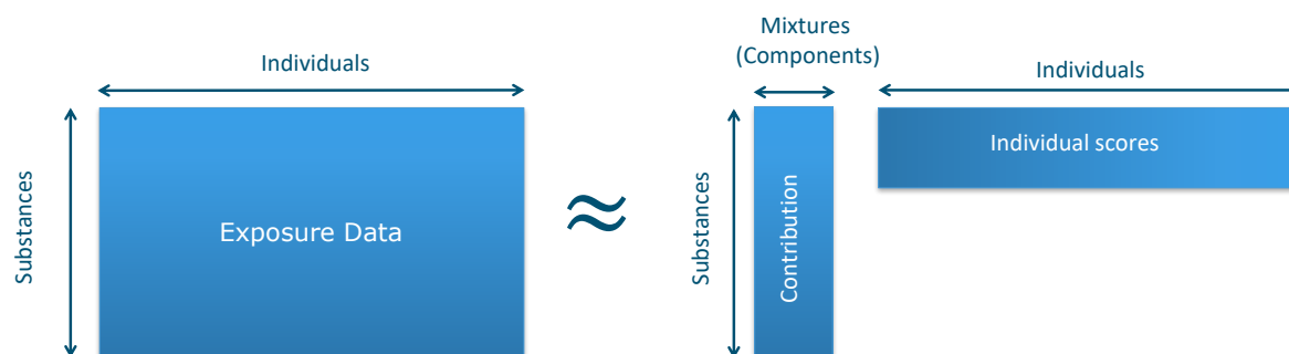
Figure 3.48: SNMU approximation of exposure data after scaling.
