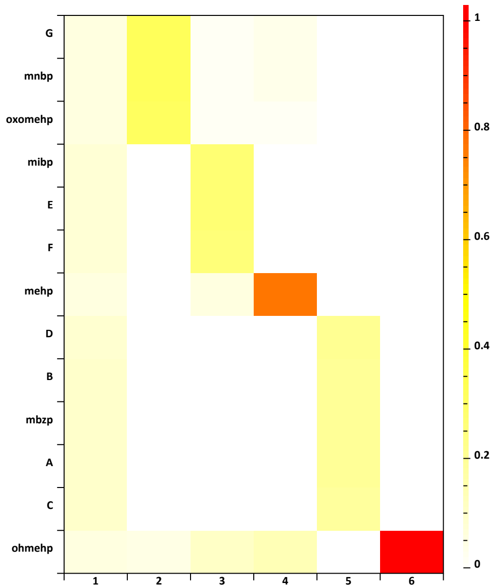
Figure 3.51: Co-exposure of substances. Heatmap for a solution with 6 components. The sparsity = 0.1. Each component, especially the first, contains many substances (see also Figure 3.52 ).
