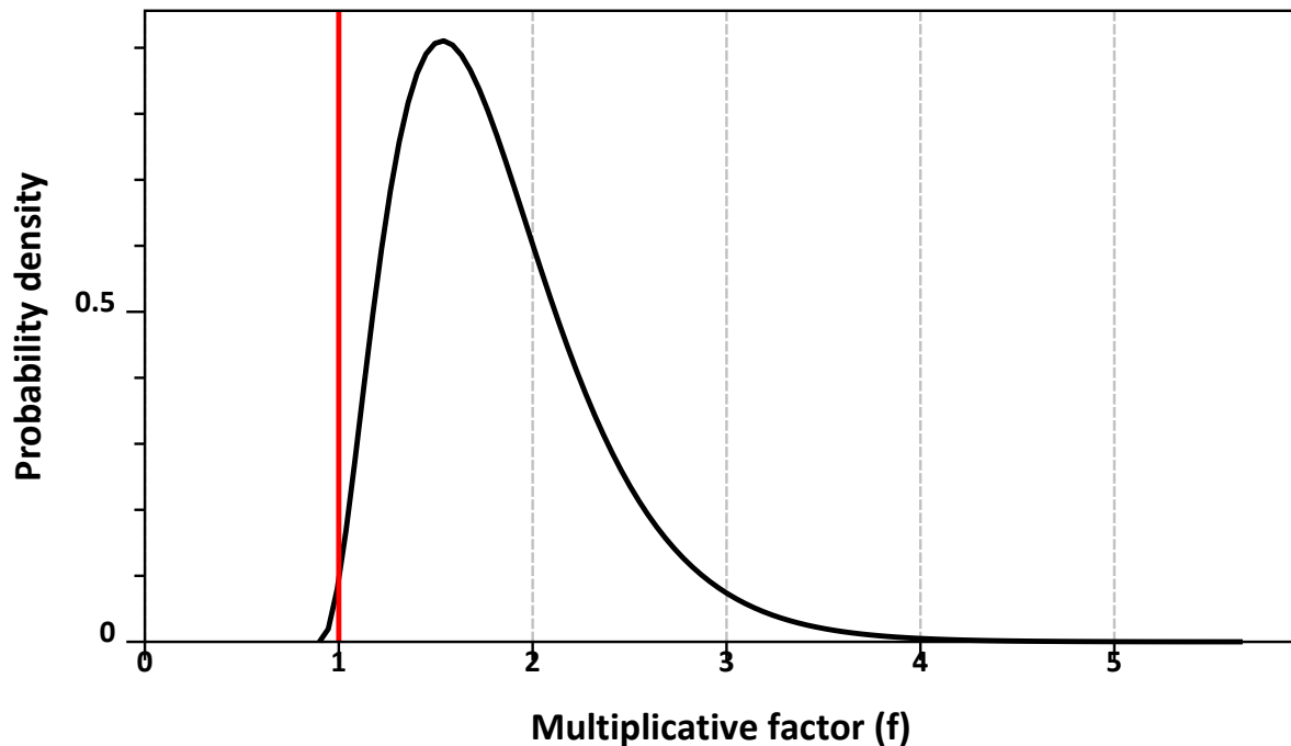
Figure 3.82: Scaled gamma ( a=3.26 , b=3.56 , \text{offset}=0.9 ), table 6, EFSA (2020a).
