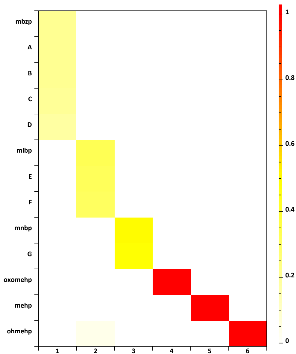
Figure 3.52: Co-exposure of substances. Heatmap for a solution with 6 components. The sparsity = 0.8. Components contain less substances compared to Figure 3.51 .
