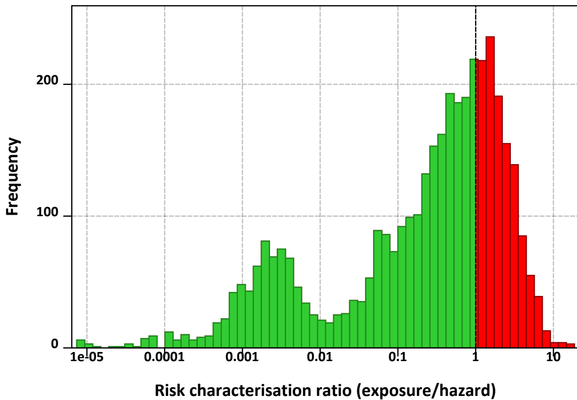
Figure 3.71: Risk characterisation ratio (exposure/hazard) based on BMDL, POCE = 32\% .
