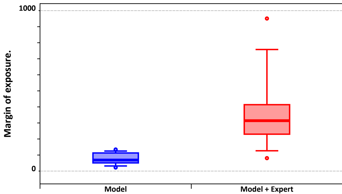
Figure 3.86: Risk characterisation ratio H/E (model) and adjusted ratio H/E (model + expert) with uncertainty bounds.
