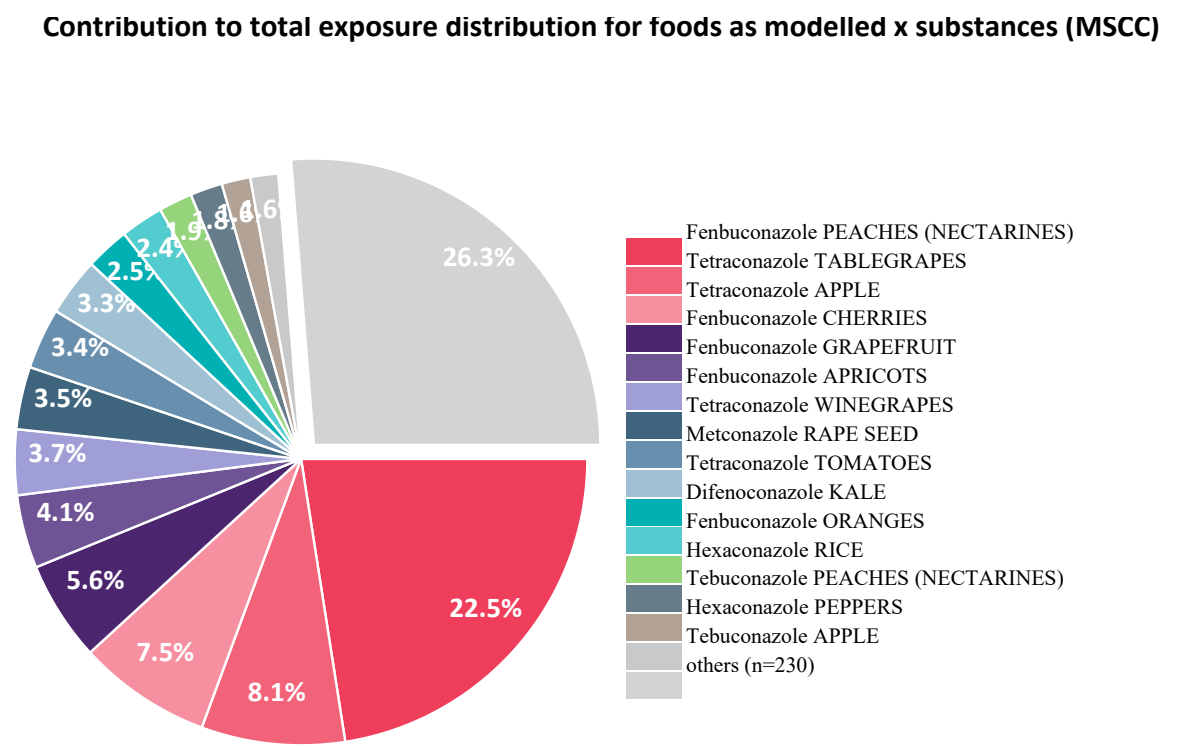
Figure 3.31: Example MCRA dietary exposure contributions substances
