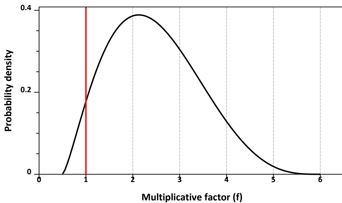
Figure 3.83: Scaled beta ( a=2.37 , b=4.26 , lowerbound=0.5, upperbound=6), table 7, EFSA (2020a) .
