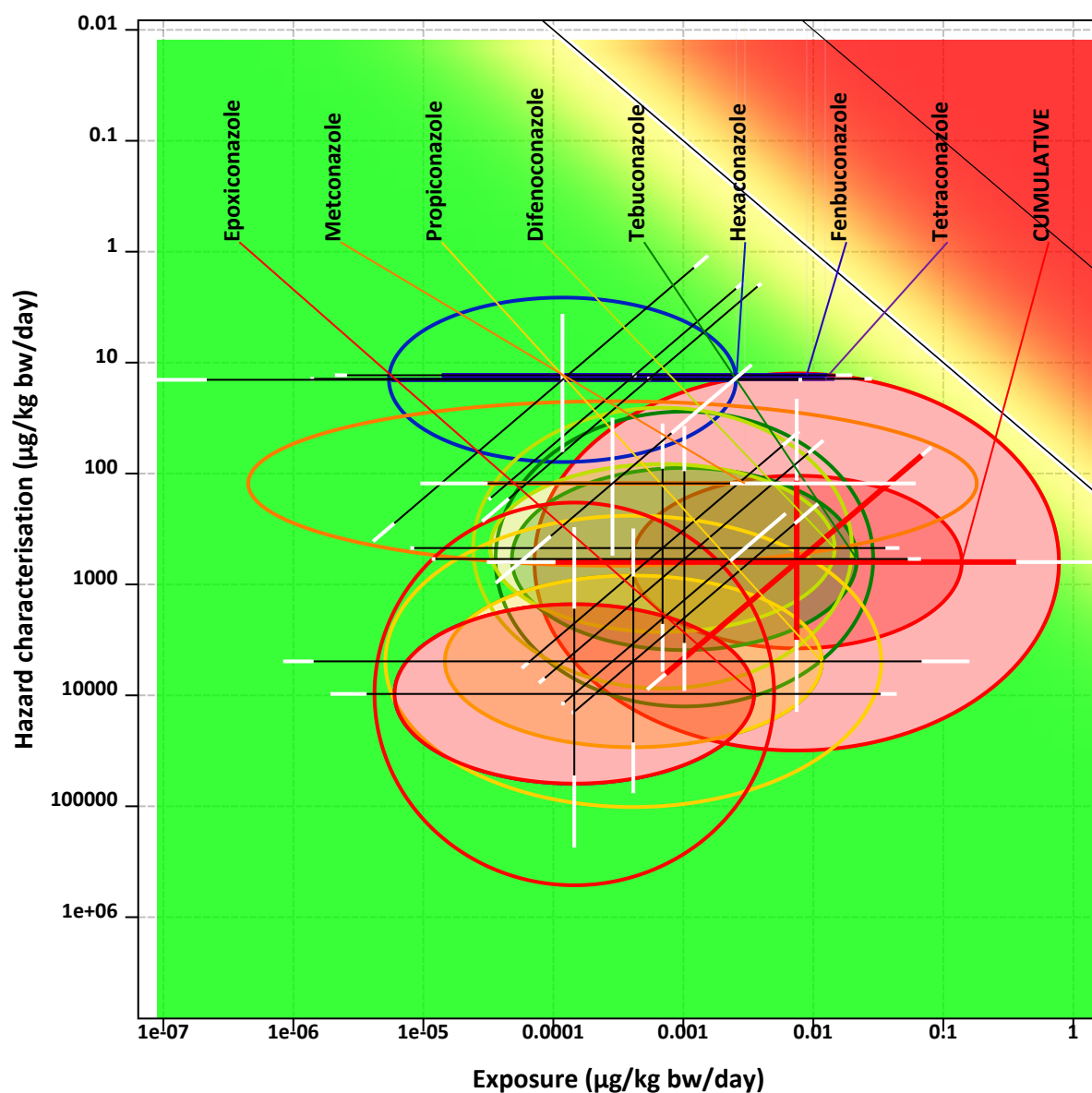
Figure 3.80: Hazard vs. exposure plot for multiple substances. 95% bivariate confidence areas for target hazard dose distribution and exposure distribution. Inner ellipses express variability, outer ellipses uncertainty.
