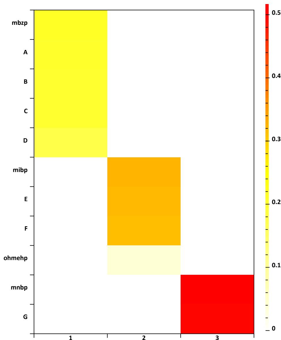
Figure 3.54: Heatmap for solution with 3 components. The first 3 components in Figure 3.54 and Figure 3.52 contain the same substances.
