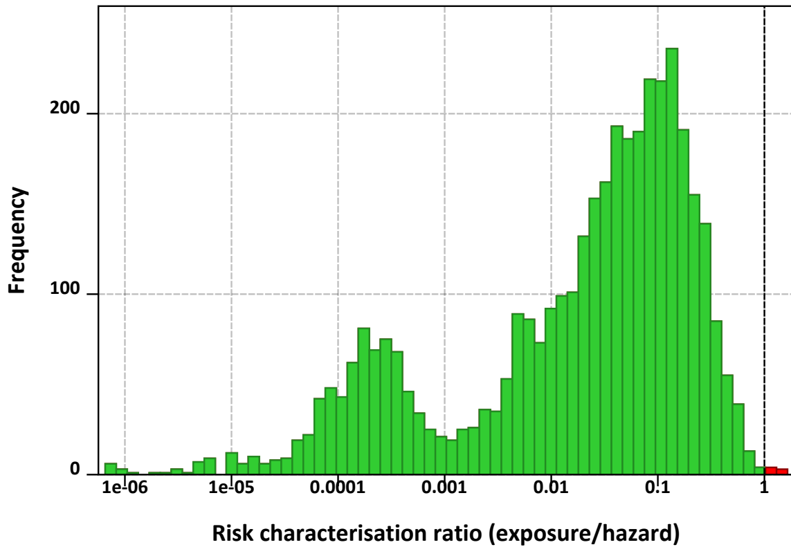
Figure 3.70: Risk characterisation ratio (exposure/hazard) based on BMD, POCE = 0.18\% .
