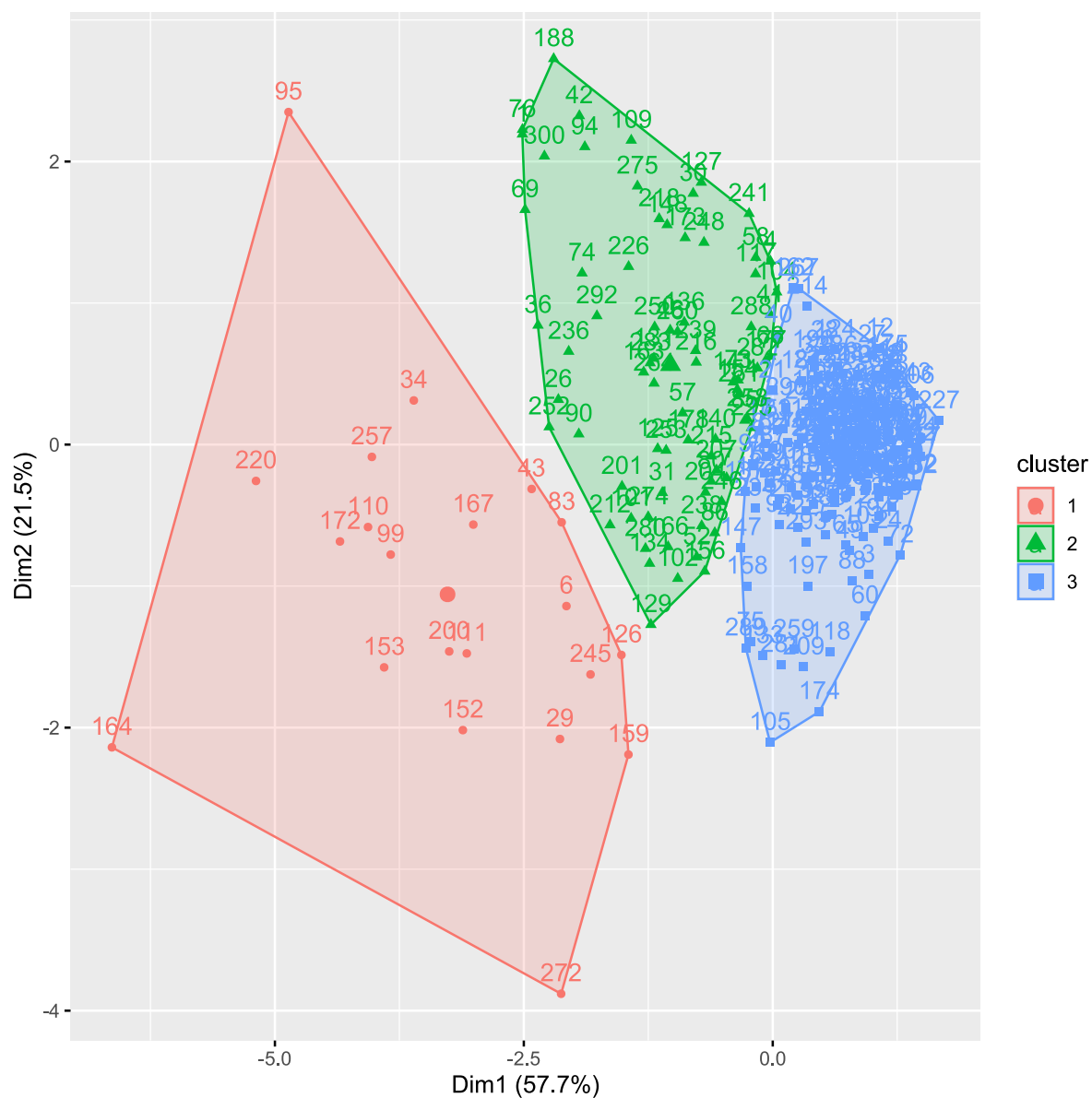
Figure 3.58: K-means clustering of human monitoring data, 3 clusters, largest and smallest cluster contain 204 and 21 individuals, respectively
