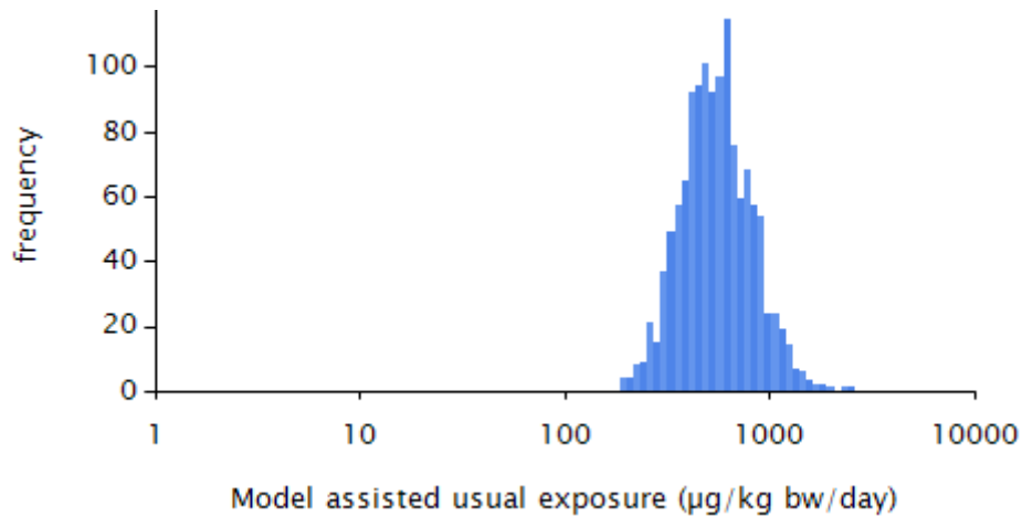
Figure 3.37: Model-based estimated usual exposure distributions (excluding the zero exposures).
