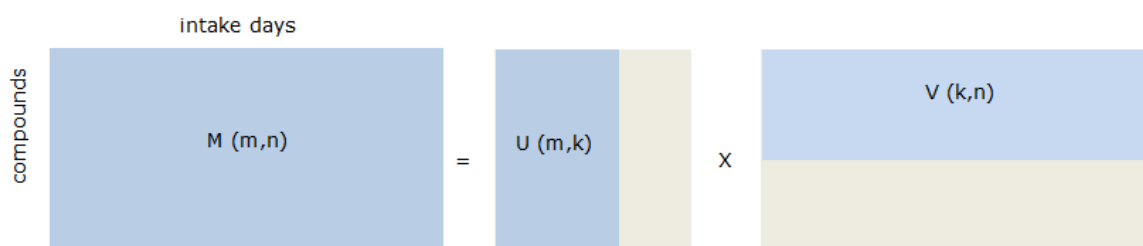
Figure 3.47: NMF approximation of exposure data
