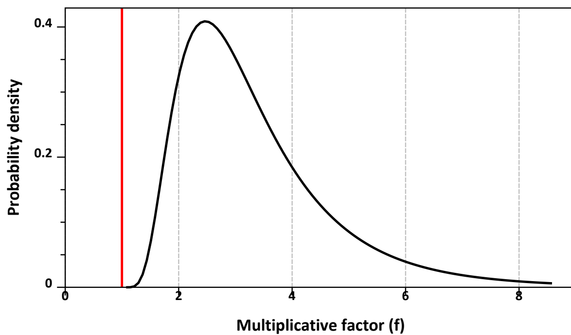
Figure 3.84: Scaled lognormal ( \mu = 0.705 , s = 0.566 , offset=1), table 8, EFSA (2020b) .
