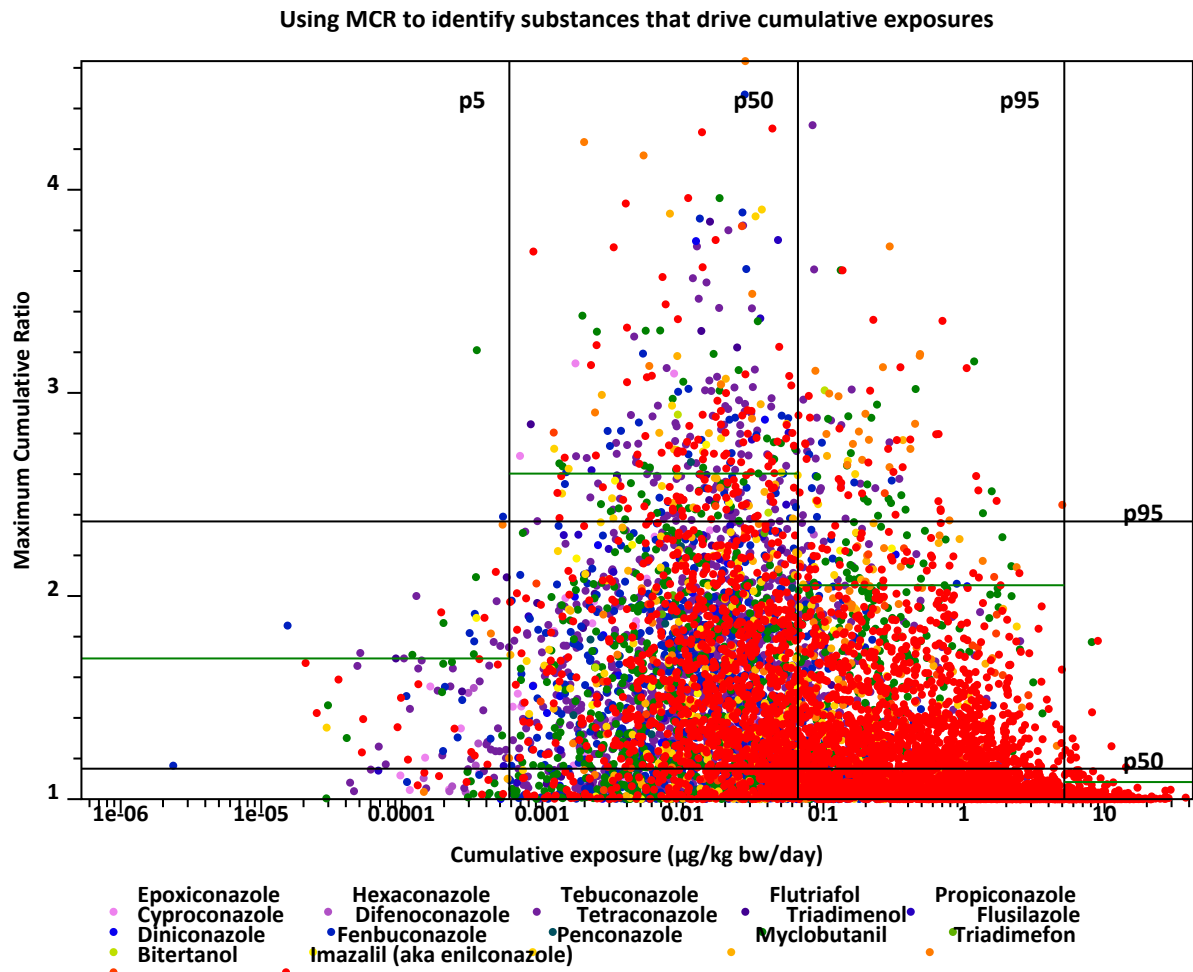
Figure 3.42: Maximum Cumulative Ratios vs total exposure
