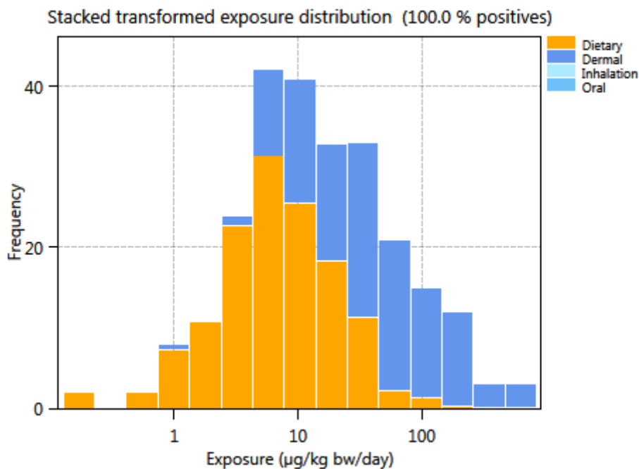
Figure 3.40: Aggregate exposure distributions.
