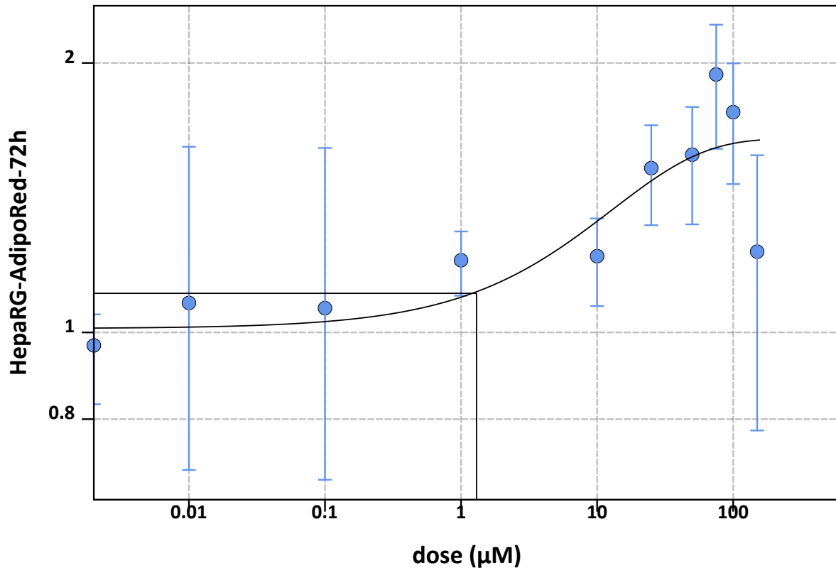
Figure 3.69: Dose response model: HepaRG Adipo72 72h.
