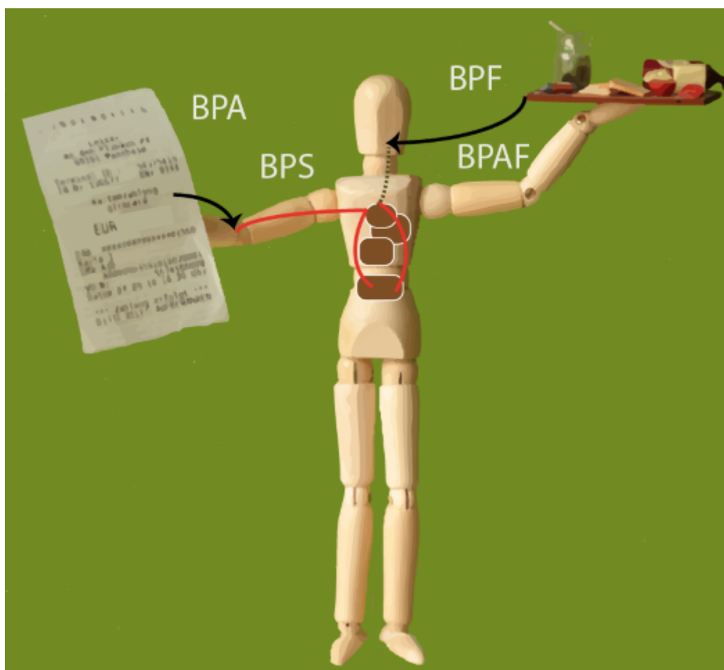
Figure 3.76: Graphical abstract 'Linking probabilistic exposure and pharmacokinetic modelling to assess the cumulative risk from the bisphenols BPA, BPS, BPF, and BPAF for Europeans.'
