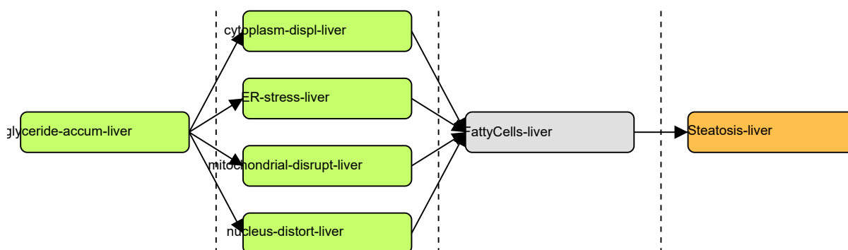
Figure 3.67: AOP network liver steatosis
