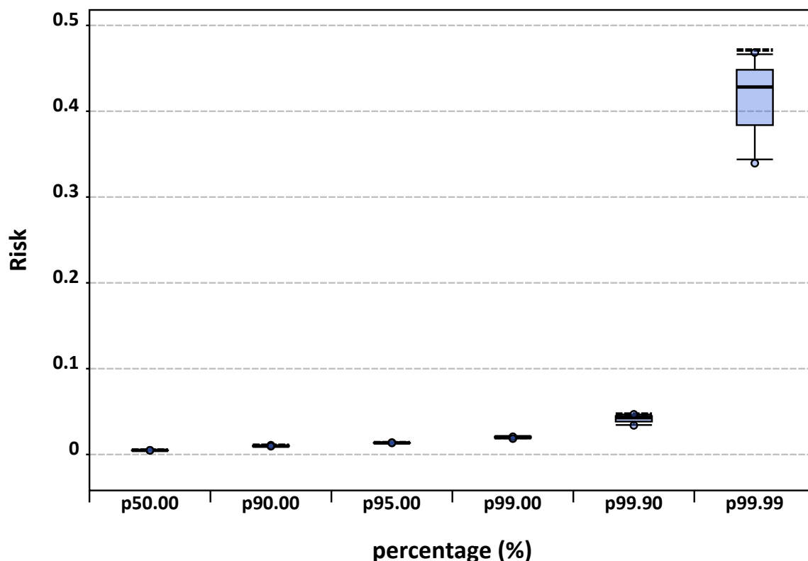
Figure 3.78: Uncertainty of percentiles. The boxplots for uncertainty show the p25 and p75 as edges of the box, and p2.5 and p97.5 as edges of the whiskers. The reference (nominal) value is indicated with the dashed black line, the median with the solid black line within the box. Outliers are displayed as dots outside the whiskers. Risk is specified as the characterisation ratio (exposure/hazard) (triazoles).
