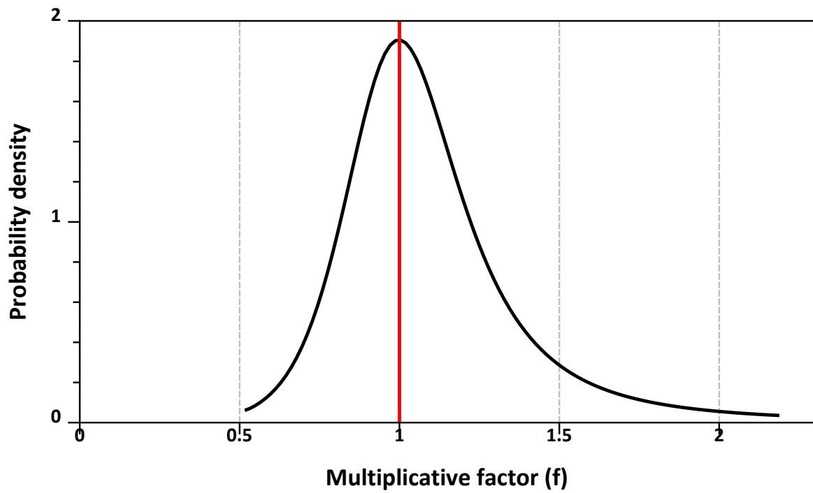
Figure 3.85: Scaled logstudent's t ( \mu = -0.593 , s = 0.367 , \nu = 3 , offset=0.5), table 9, EFSA (2020b) .
