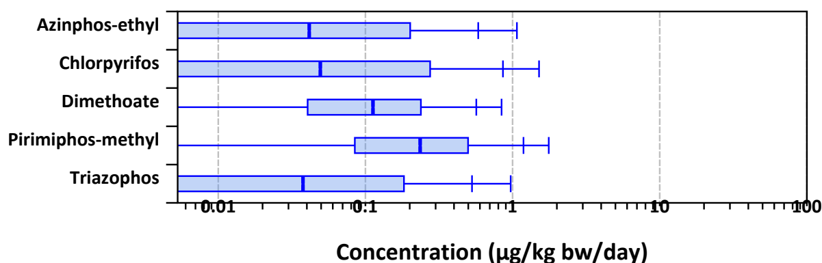
Figure 3.64: Boxplots for imputed concentration data for five pesticides. Lower whiskers indicate the p5 and p10 percentiles, upper whiskers the p90 and p95. The edges of the box indicate the p25 and p75 percentiles with the median in the centre of the box.
