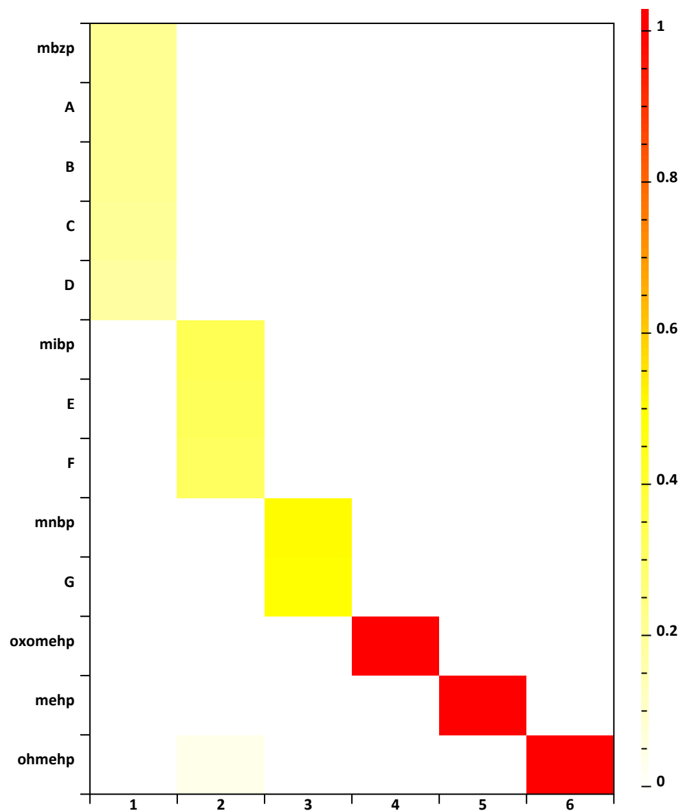
Figure 3.60: SNMU solution with 6 components. Sparsity = 0.8.
