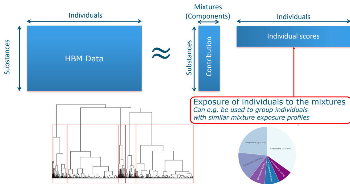
Figure 3.55: SNMU: matrix V , individual scores to components.
