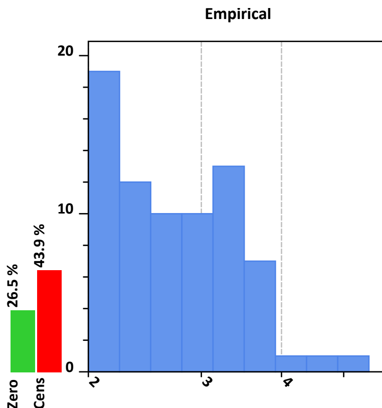
Figure 3.16: Empirical distribution
