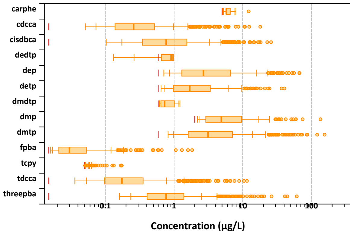
Figure 3.65: Boxplots for positive/quantified HBM substance concentration measurements of 13 pesticides. Lower whiskers indicate the p5 and p10 percentiles, upper whiskers the p90 and p95. The edges of the box indicate the p25 and p75 percentiles and the median in the centre of the box. LORs are displayed by a vertical red bar and outliers outside range ( Q1 - 3 * IQR , Q3 + 3 * IQR ).
