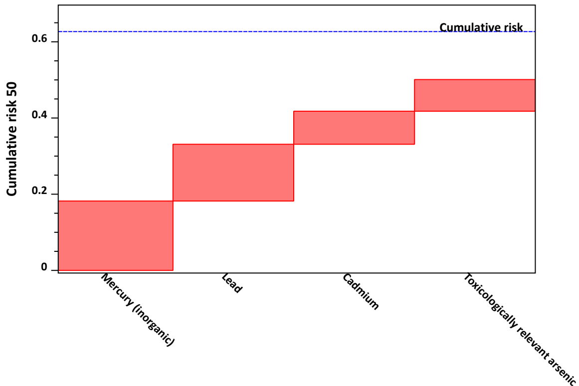
Figure 3.81: Cumulative risk characterisation ratios exposure/hazard (median) in the population (metals).
